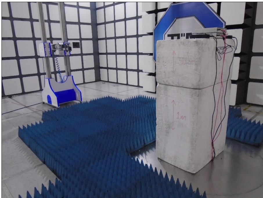
Figure 2 – Radiated Disturbance - 1 GHz to 10 GHz
