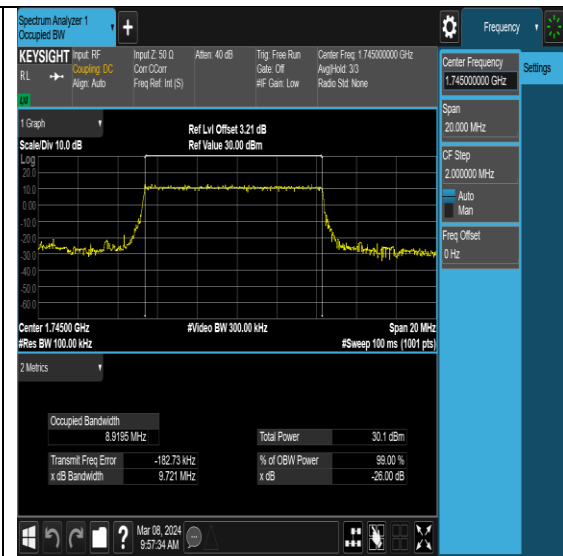
NTNV-N66-PC3-15-10-M-DFT-PI2BPSK-Outer_Full-Ant0-PASS
