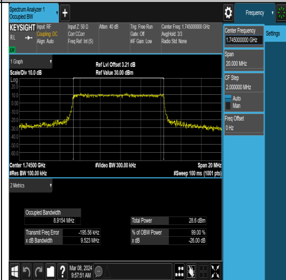
NTNV-N66-PC3-15-10-M-DFT-16QAM-Outer_Full-Ant0-PASS
