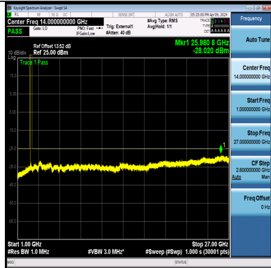
NTVN-N41-PC2-30-100-H-CP-QPSK- Edge_1RB_Left-Ant0-PASS
