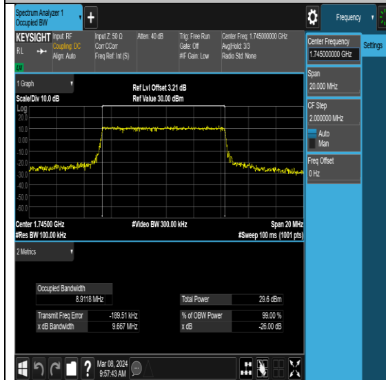
NTNV-N66-PC3-15-10-M-DFT-QPSK-Outer_Full-Ant0-PASS
