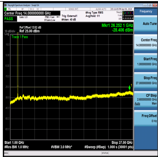
NTVN-N41-PC2-30-100-H-CP-QPSK- Edge_1RB_Left-Ant2-PASS
