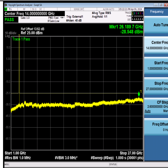
NTNV-N41-PC2-30-20-H-CP-QPSK- Edge_1RB_Left-Ant0-PASS
