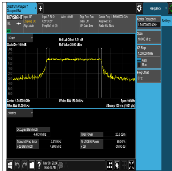
NTNV-N66-PC3-15-5-M-DFT-256QAM-Outer_Full-Ant0-PASS
