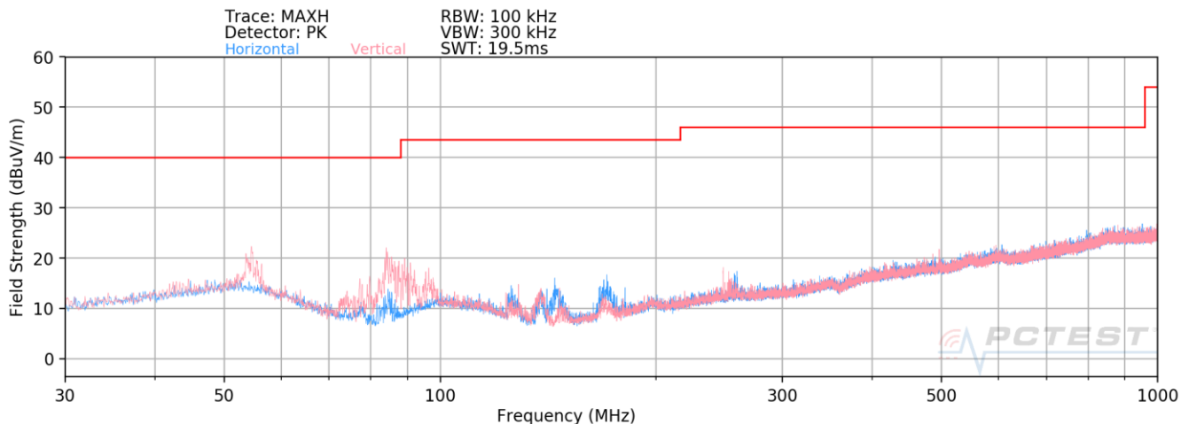
Plot 7-3. Radiated Spurious Plot below 1GHz Case #3
