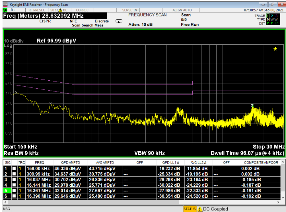
Plot 7-5. Line Conducted Plot (N)
