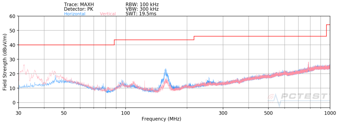
Plot 7-2. Radiated Spurious Plot below 1GHz Case #2
