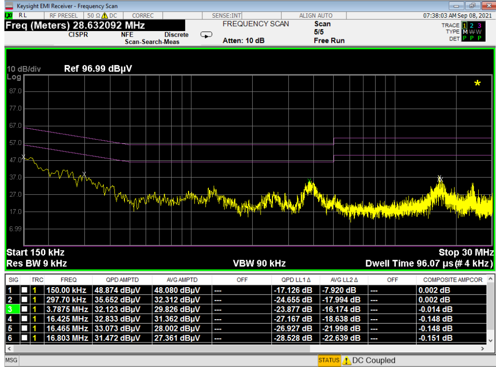
Plot 7-4. Line Conducted Plot (L1)
