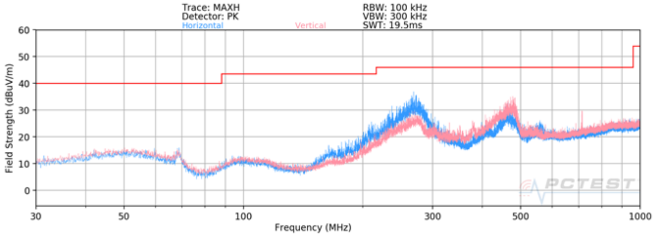
Plot 7-1. Radiated Spurious Plot below 1GHz Case #1
