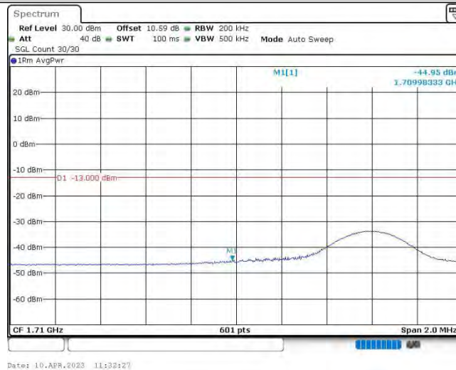
Band4-10MHz-16QAM-20000-1RB#49
