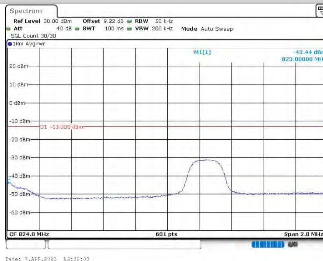
Band5-3MHz-QPSK-20415-1RB#14
