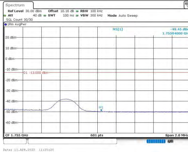
Band4-5MHz-16QAM-20375-1RB#0
