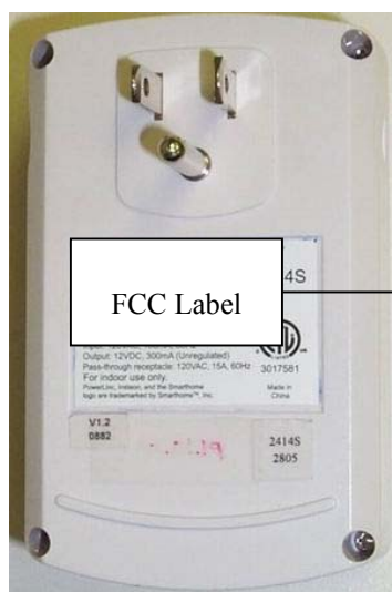
Figure 2.2 FCC ID Label Location
