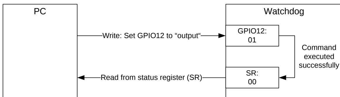
Figure 18: Write data to address register
