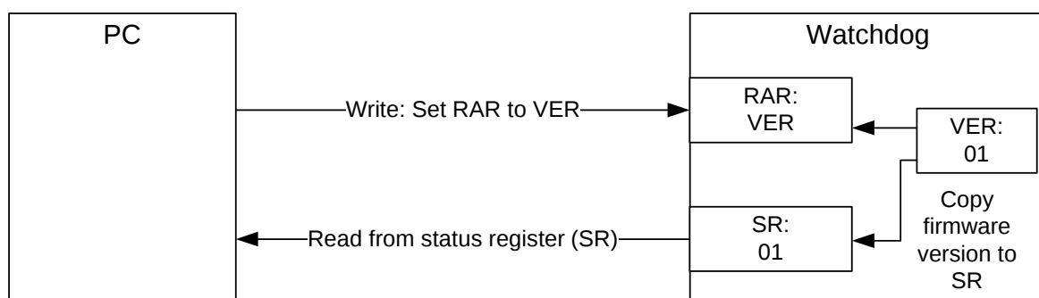
Figure 19: Read data from address register
