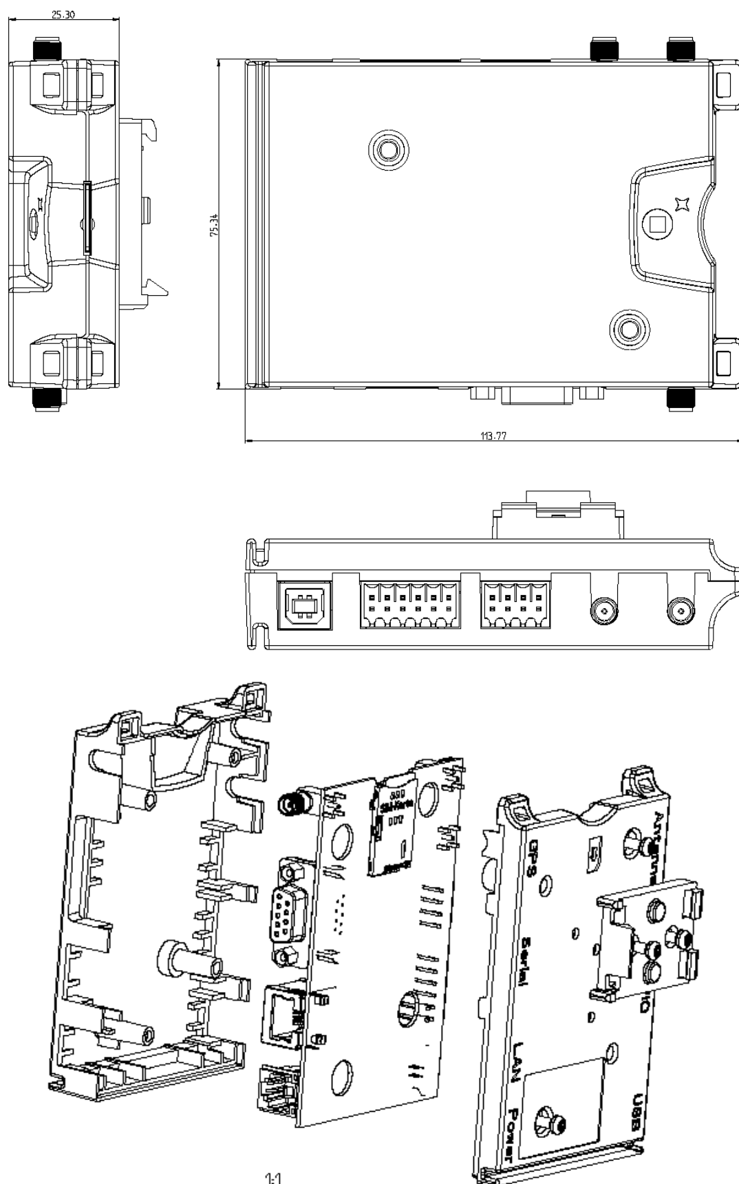
Figure 14: Java Terminals mechanical dimensions
