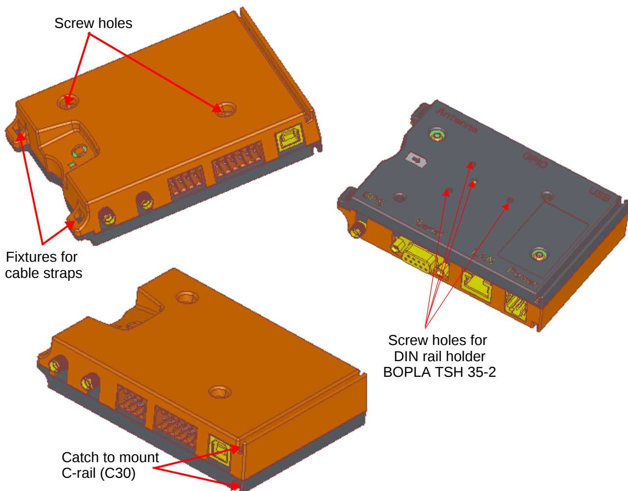
Figure 15: Mounting the Java Terminals
