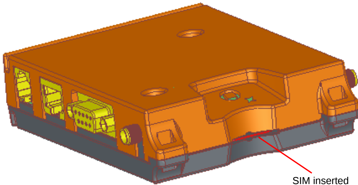
Figure 10: SIM interface
