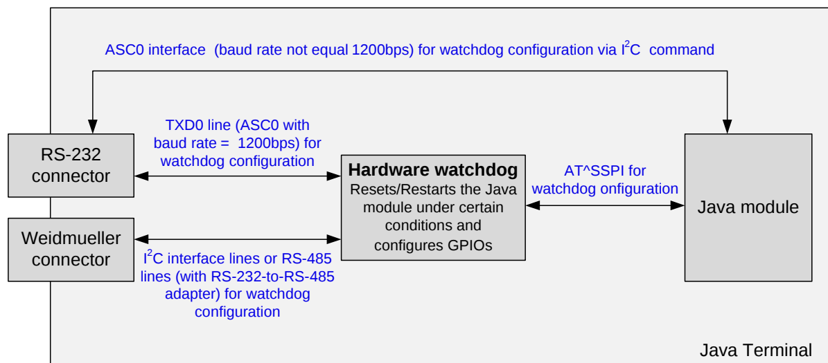
Figure 17: Hardware watchdog
