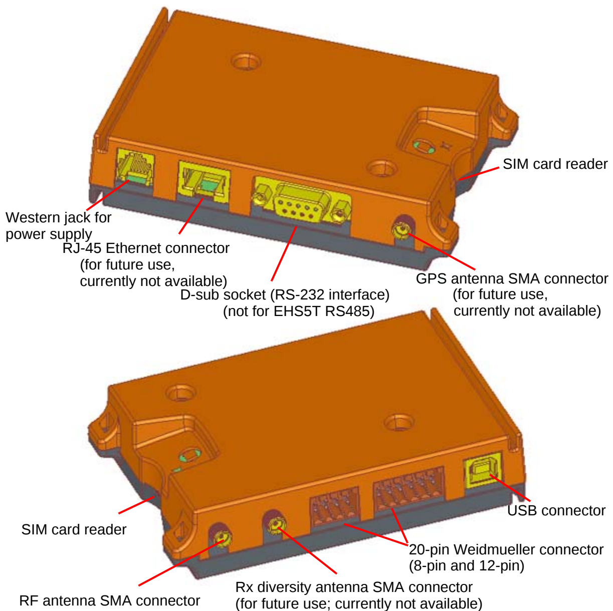
Figure 2: Java Terminals 3D view
