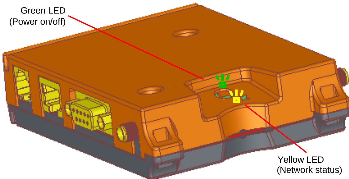
Figure 11: Status LED
