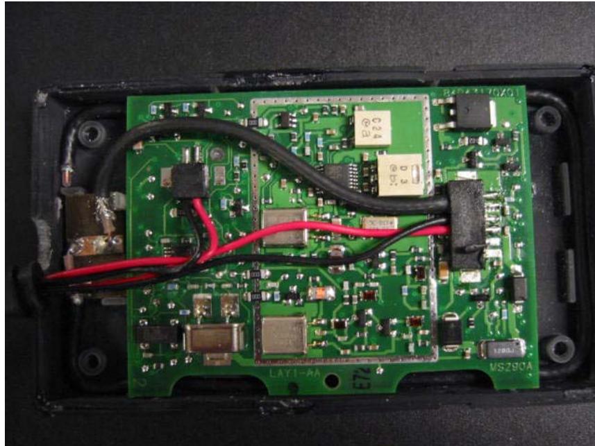
Internal Photographs FCC ID: IDILJU-03U
