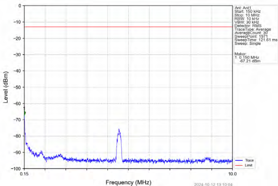
Band66_10MHz_16QAM_LCH_1715MHz_RB_1_0_NTNV
