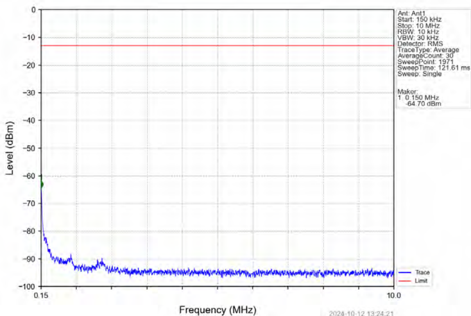
Band66_15MHz_16QAM_MCH_1745MHz_RB_1_0_NTNV
