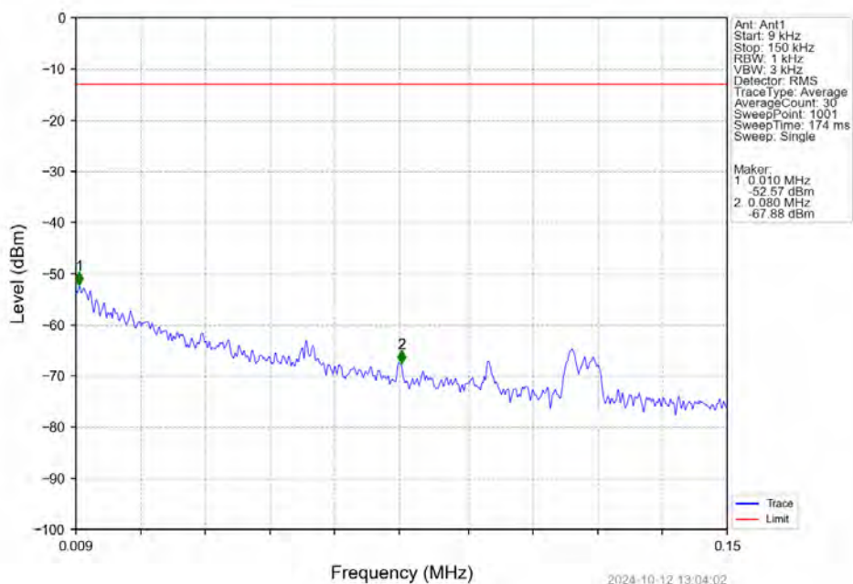
Band66_5MHz_16QAM_HCH_1777.5MHz_RB_1_0_NTNV
