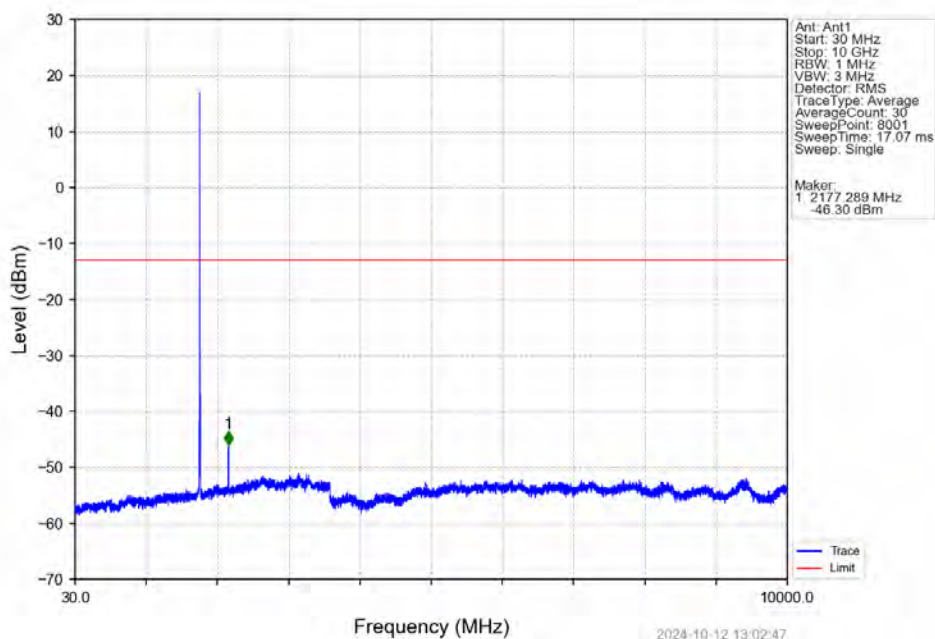
Band66_5MHz_QPSK_HCH_1777.5MHz_RB_1_0_NTV
