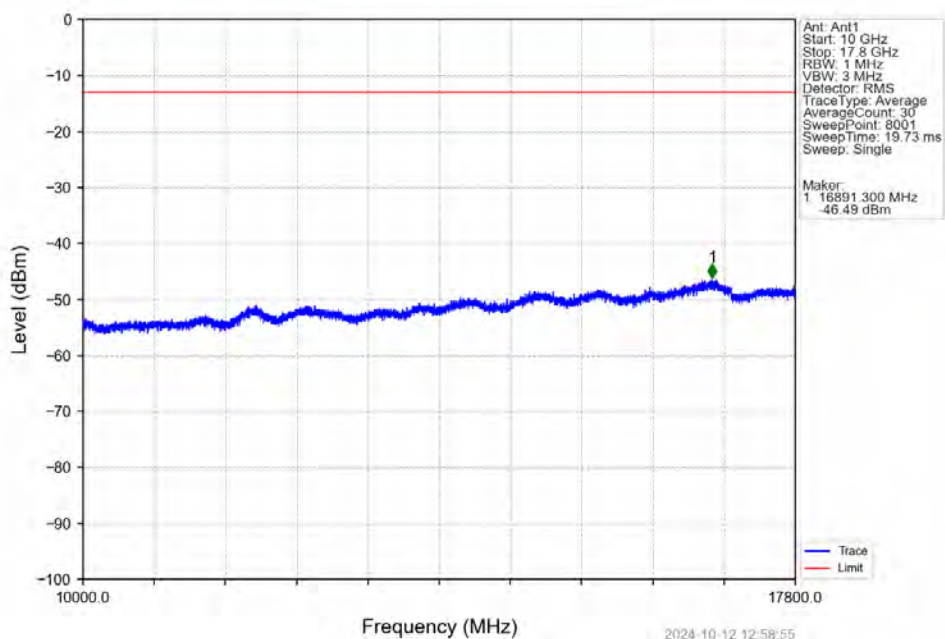
Band66_5MHz_QPSK_LCH_1712.5MHz_RB_1_0_NTNV
