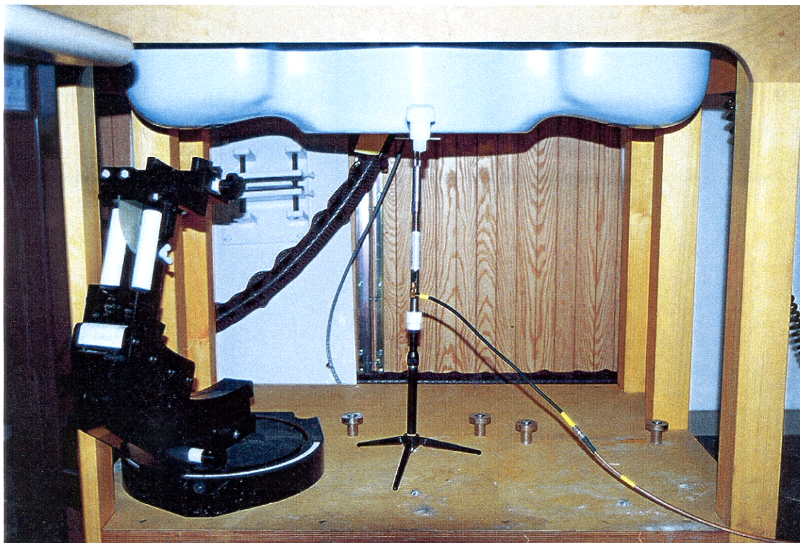
Photo 6 – Validation Dipole Set-up
