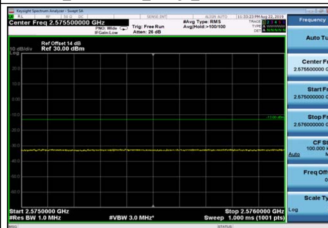
FDD07_15MHz_2562.5_QPSK_fullRB _ExtraBands_Range_2575~2576
