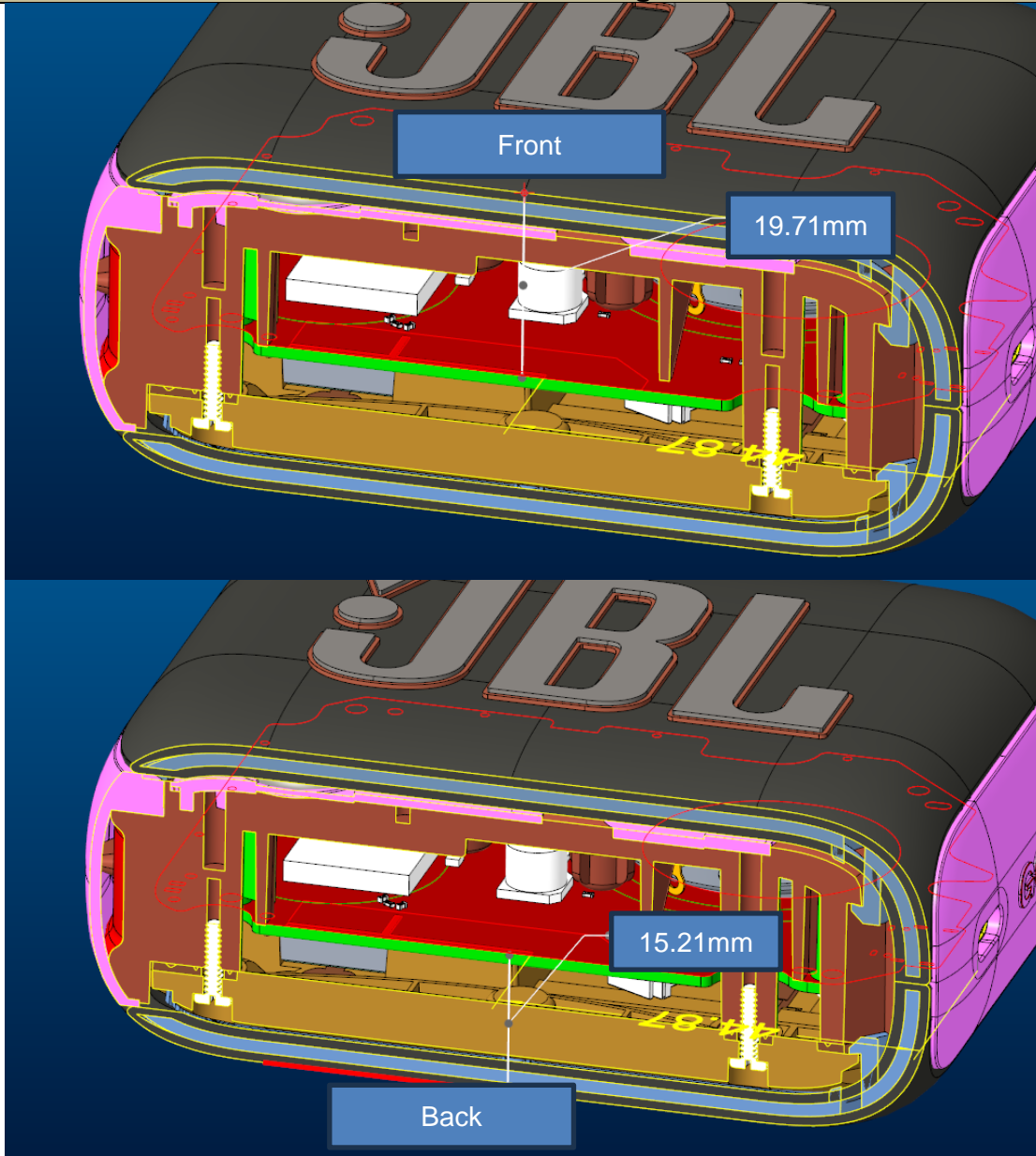
Antenna location diagram
