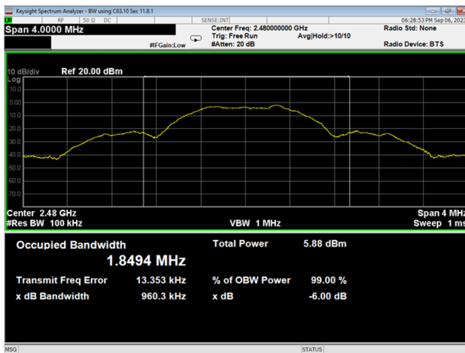
06 6dB Bandwidth, High Channel, GFSK
