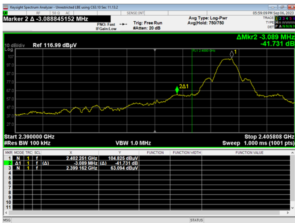
23 Lower Bandedge, Unrestricted, GMSK 1MB
