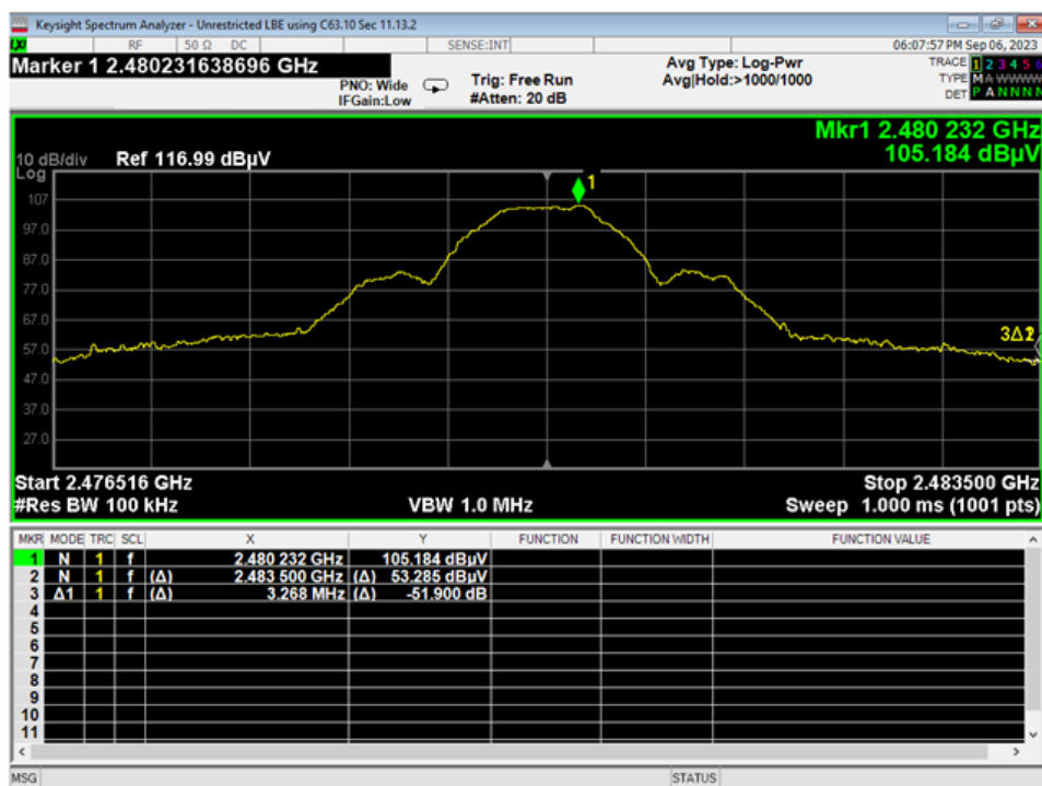
24 Higher Bandedge, Unrestricted, GMSK 1MB
