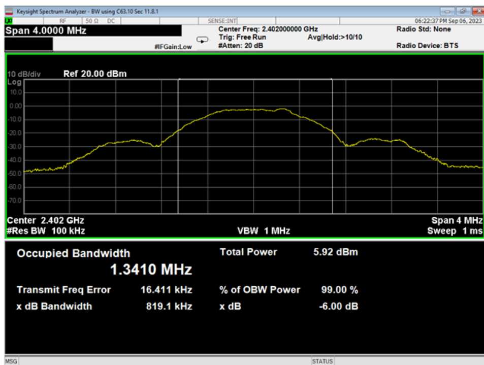
04 6dB Bandwidth, Low Channel, GFSK
