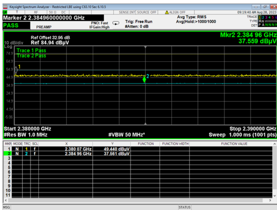
25 Lower Bandedge, Restricted, GMSK 1MB
