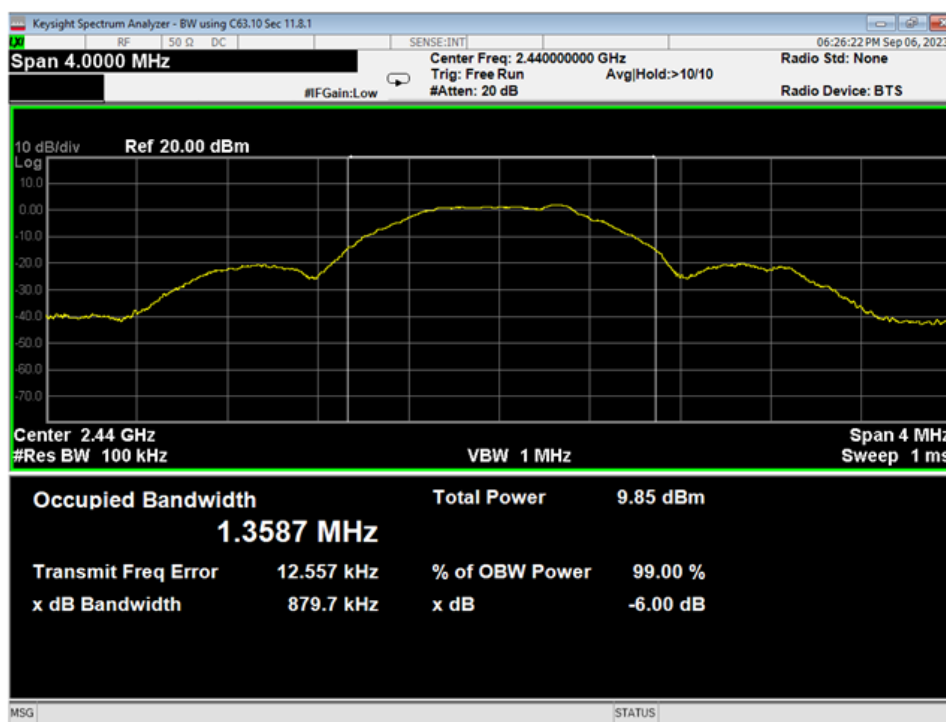
05 6dB Bandwidth, Mid Channel, GFSK
