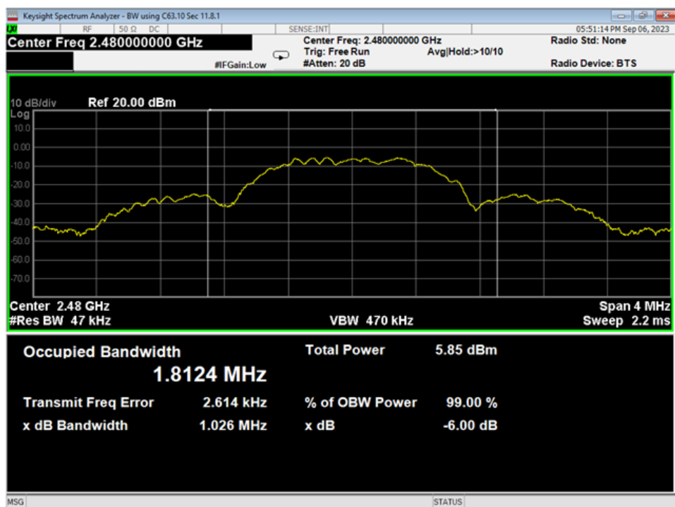
42 Occupied Bandwidth, High Channel, GFSK
