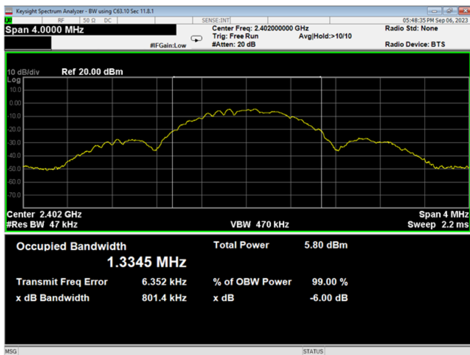
40 Occupied Bandwidth, Low Channel, GFSK
