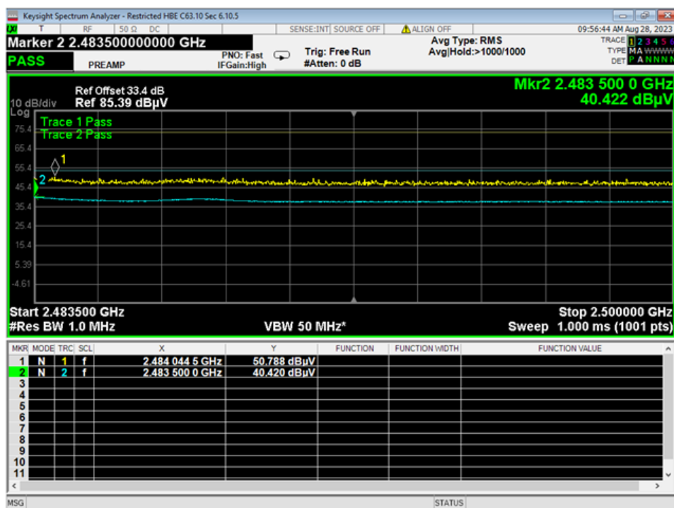
26 Higher Bandedge, Restricted, GMSK 1MB
