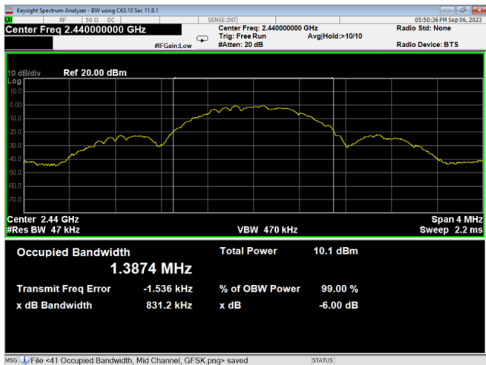
41 Occupied Bandwidth, Mid Channel, GFSK
