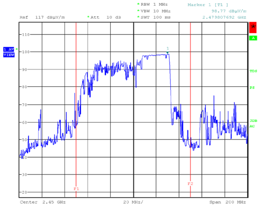
< Fig 9. Frequency Measurements _Load (Maximum Frequency Observed: 2.479 GHz) >
