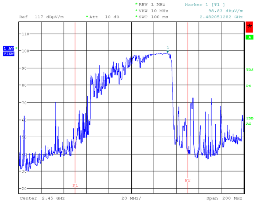
< Fig 7. Frequency Measurements _ Voltage (Maximum Frequency Observed: 2.482 GHz) >
