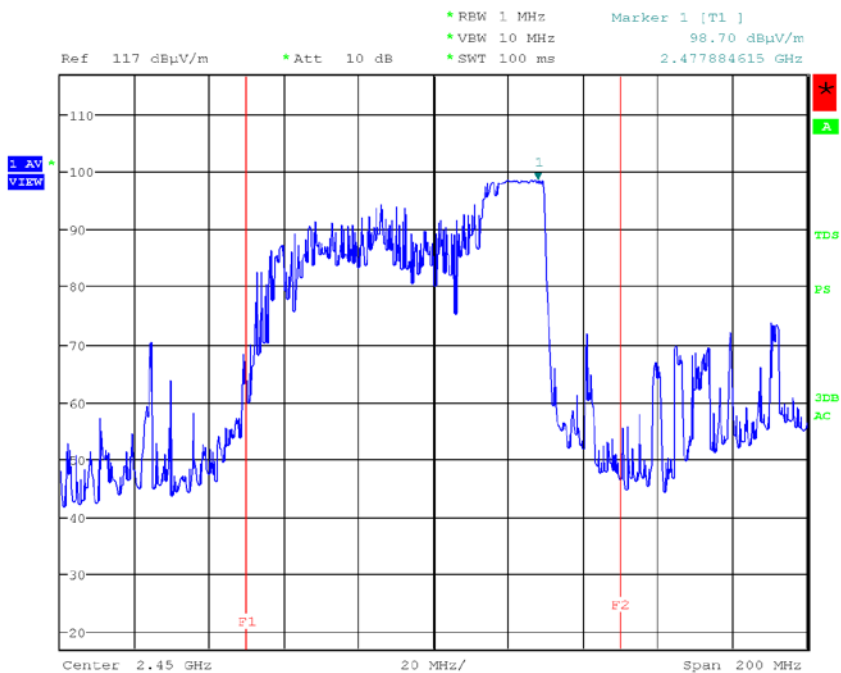
< Fig 10. Frequency Measurements _Load (Minimum Frequency Observed: 2.477 GHz) >
