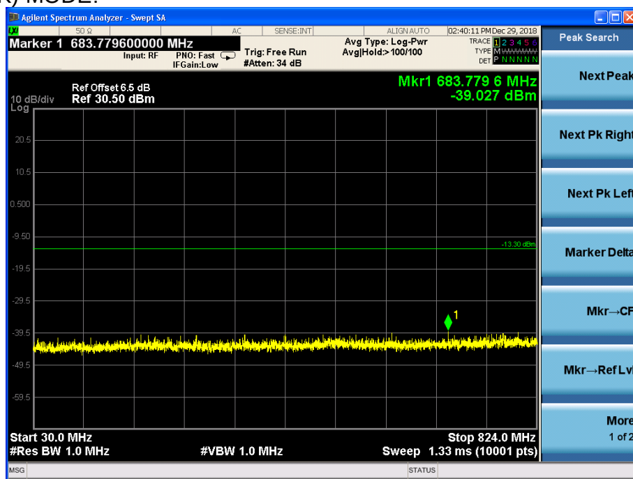
Channel 189, 30MHz~824MHz
