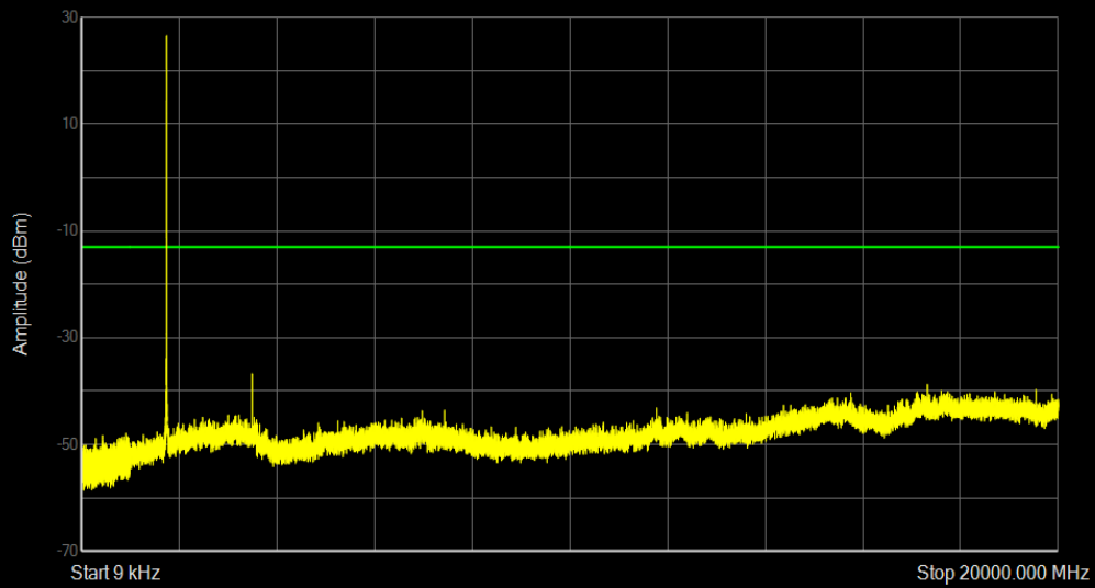
Band4 16QAM BW=3MHz Channel=20385 RB Size=1 Position=#0
