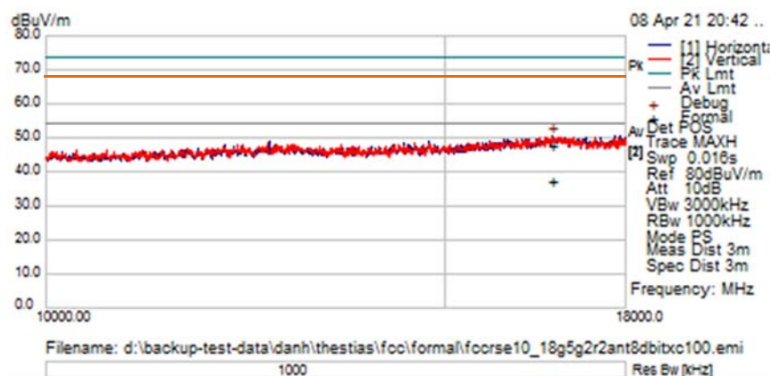
TX Spurious Emissions from 10GHz-18GHz – Ch100 (5500 MHz)
