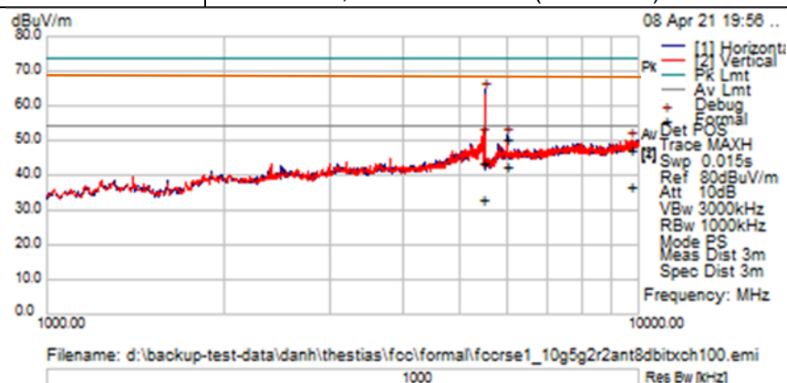
TX Spurious Emissions from 1GHz-10GHz – Ch100 (5500 MHz)
