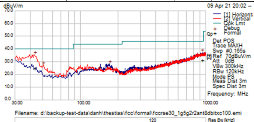
TX Spurious Emissions from 30MHz-1GHz – Ch100 (5500 MHz)
