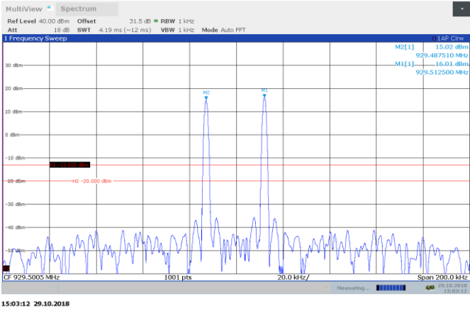
Figure 8.5-1: 929.4875 and 929.5125 MHz AGC + 0.5 Out-of-block
