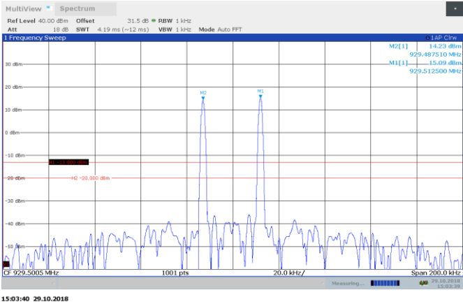
Figure 8.5-2: 929.4875 and 929.5125 MHz AGC + 3dB Out-of-block
