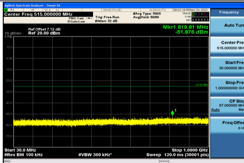
Band7-5MHz-QPSK-21425-1RB#0-30~1000MHz
