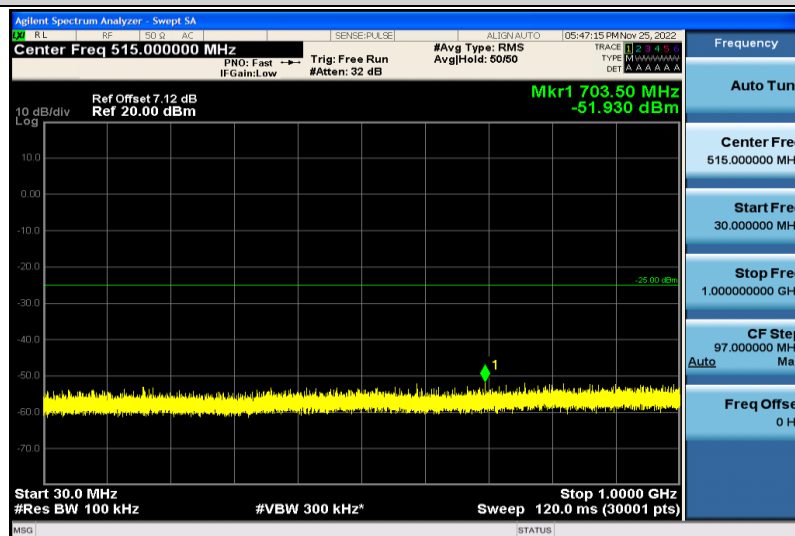
Band7-10MHz-64QAM-21400-1RB#0-30~1000MHz
