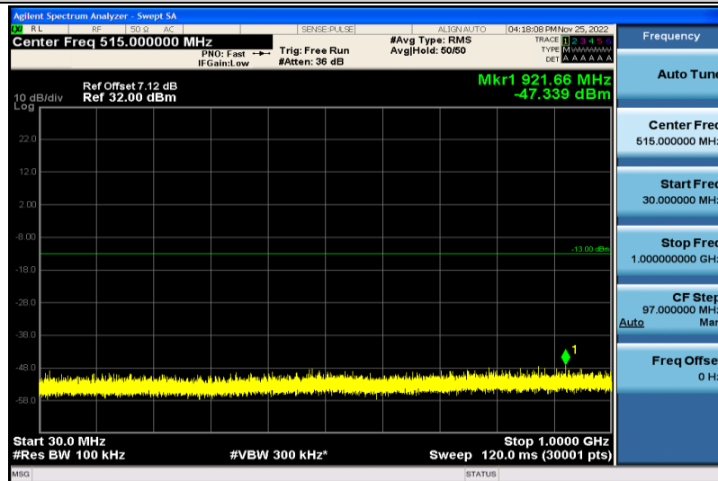
Band4-10MHz-64QAM-20350-1RB#0-30~1000MHz
