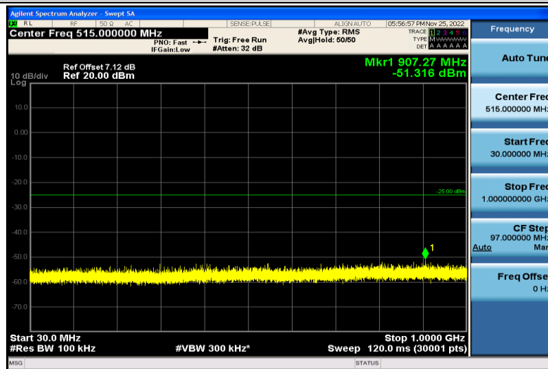
Band7-15MHz-64QAM-20825-1RB#0-30~1000MHz
