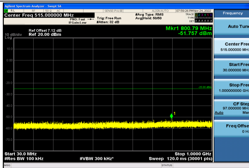
Band7-5MHz-16QAM-20775-1RB#0-30~1000MHz
