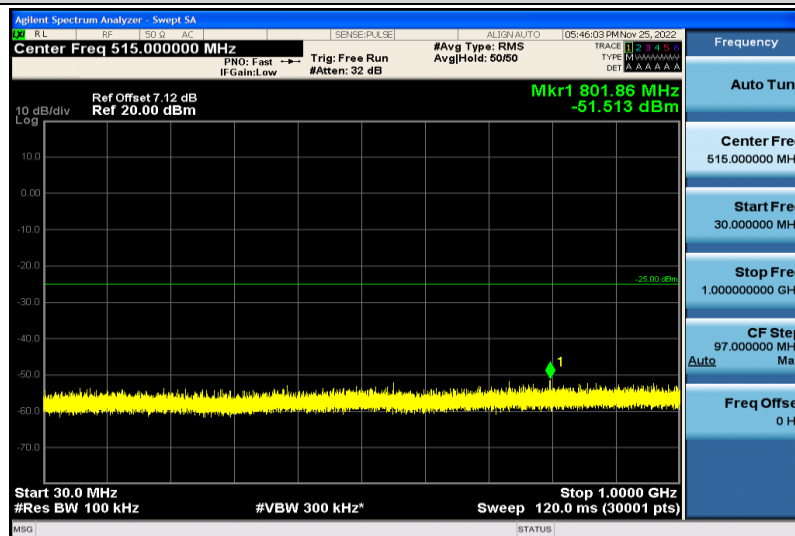
Band7-10MHz-64QAM-20800-1RB#0-30~1000MHz
