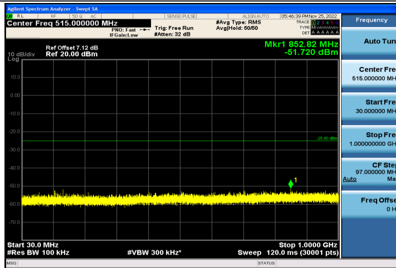
Band7-10MHz-64QAM-21100-1RB#0-30~1000MHz
