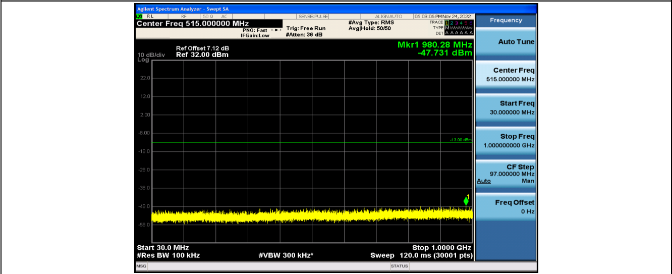
Band4-15MHz-QPSK-20025-1RB#0-30~1000MHz
