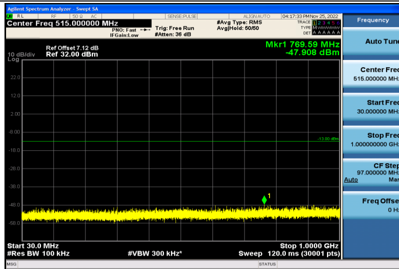
Band4-10MHz-64QAM-20175-1RB#0-30~1000MHz
