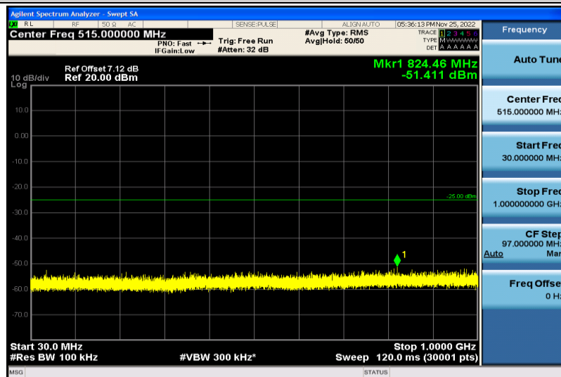
Band7-5MHz-64QAM-20775-1RB#0-30~1000MHz
