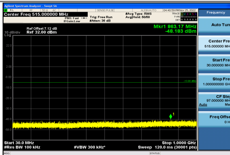
Band4-20MHz-64QAM-20300-1RB#0-30~1000MHz
