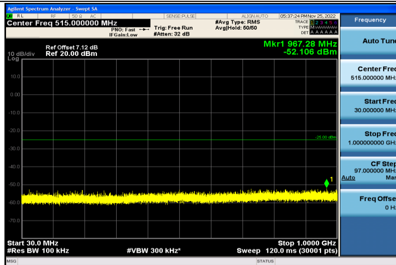
Band7-5MHz-64QAM-21425-1RB#0-30~1000MHz
