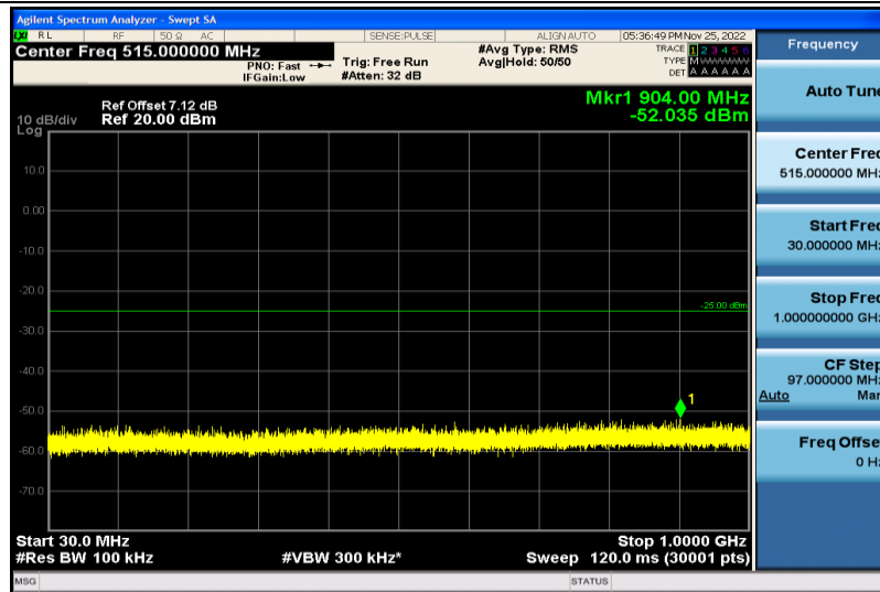
Band7-5MHz-64QAM-21100-1RB#0-30~1000MHz
