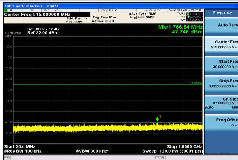
Band4-10MHz-64QAM-20000-1RB#0-30~1000MHz
