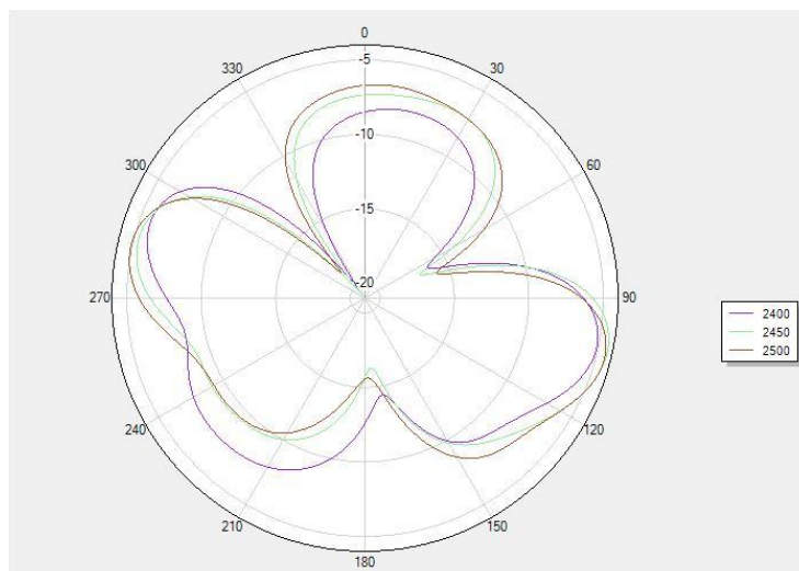
Theta 90 2D
