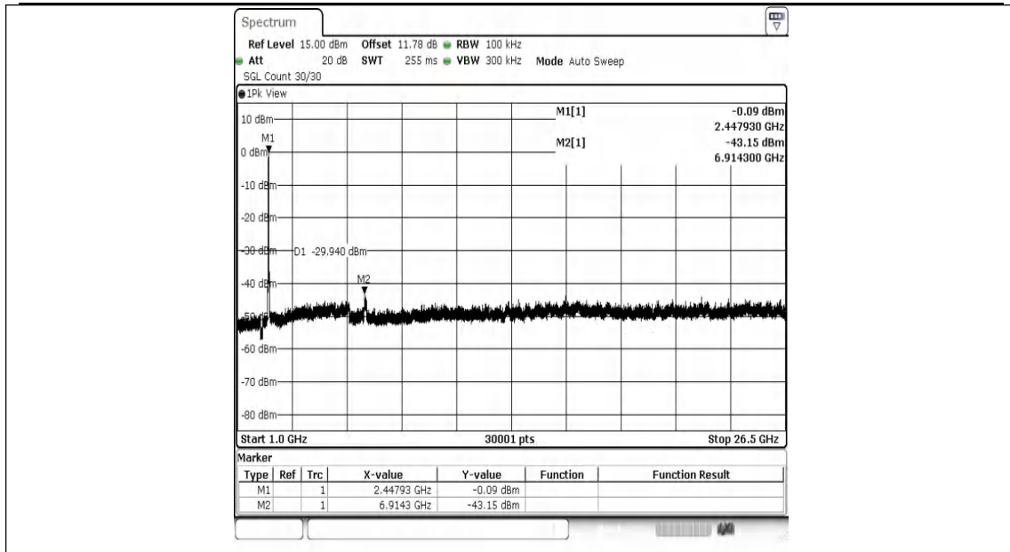
11N40SISO-Ant1-2437-1000~26500-PASS
