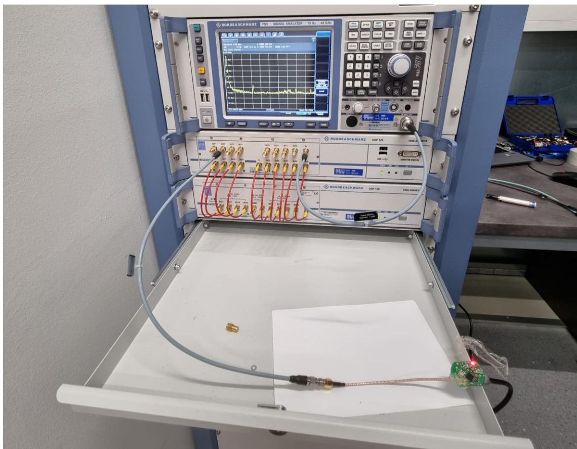
Figure 6: Conducted measurements test setup
