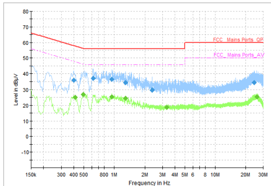
Fig.69 AC Power line Conducted Emission (Traffic, AE3, 120V)
