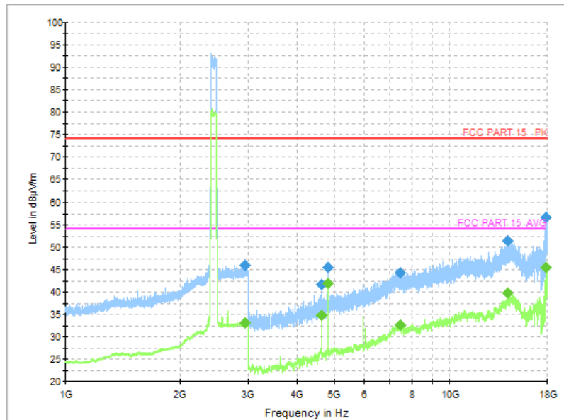
Fig.45 Radiated Spurious Emission (802.11b, CH1, 1GHz-18GHz)
