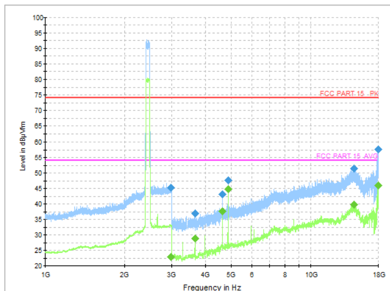
Fig.46 Radiated Spurious Emission (802.11b, CH6, 1GHz-18GHz)
