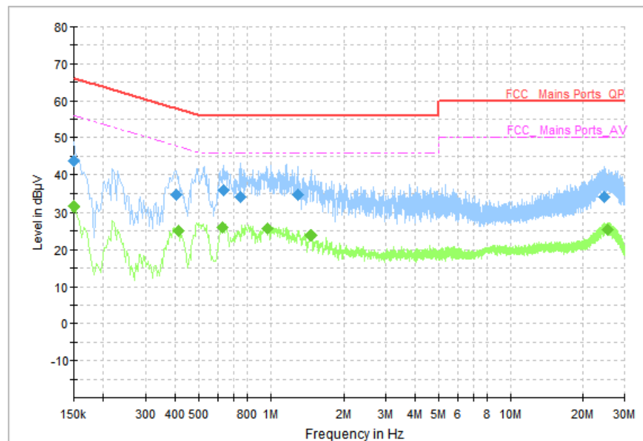
Fig.68 AC Power line Conducted Emission (Idle, AE3, 120V)
