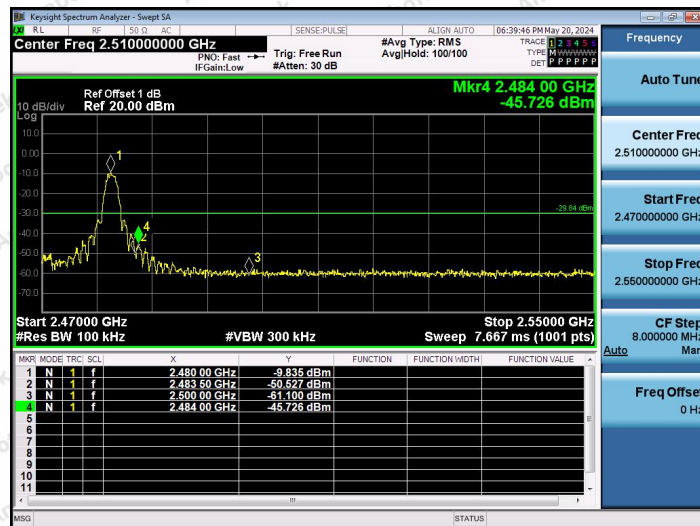
Zigbee-Ant1-2480-PASS
