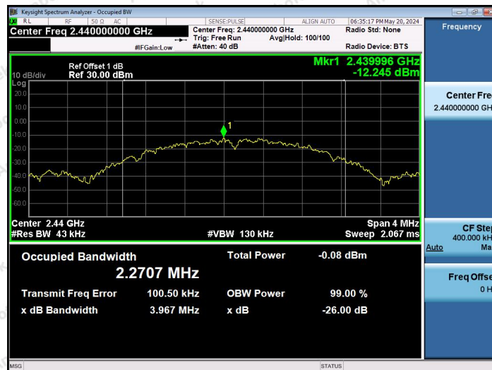
Zigbee-Ant1-2440
