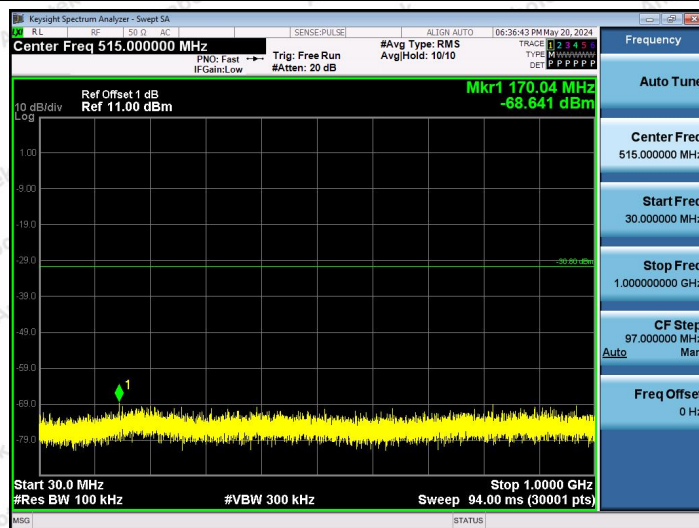
Zigbee-Ant1-2440-30~1000-PASS
