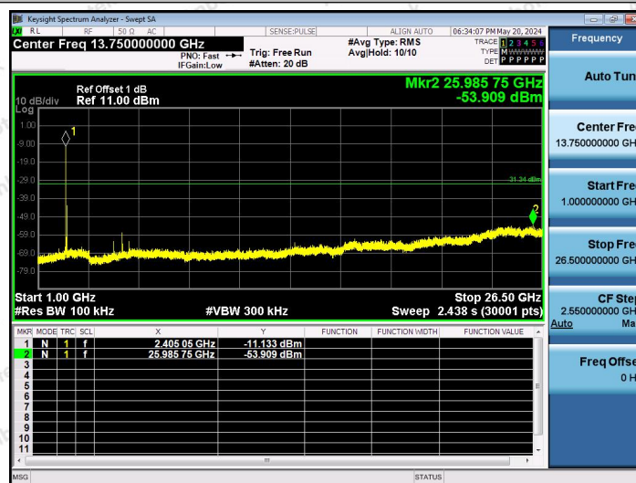
Zigbee-Ant1-2405-1000~26500-PASS
