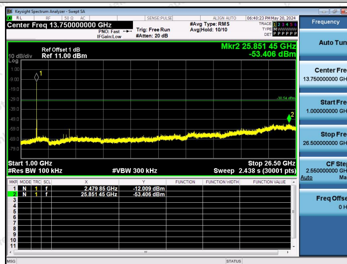
Zigbee-Ant1-2480-1000~26500-PASS
