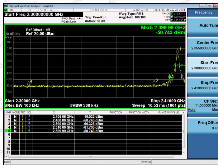
Zigbee-Ant1-2405-PASS
