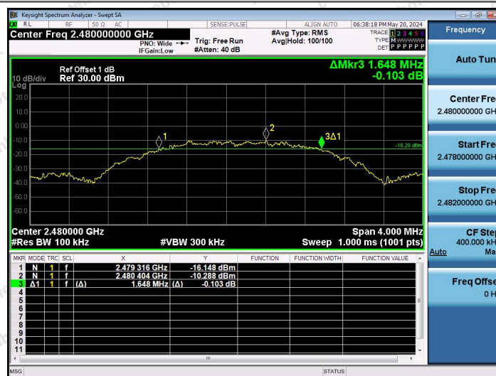
Zigbee-Ant1-2480-PASS
