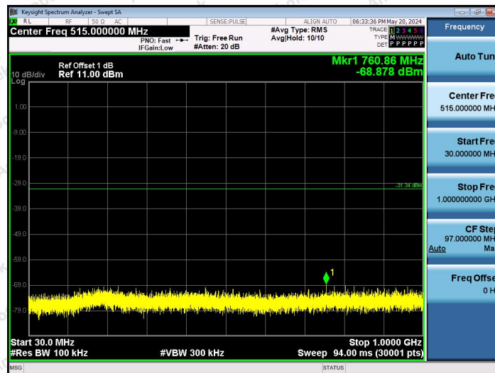
Zigbee-Ant1-2405-30~1000-PASS
