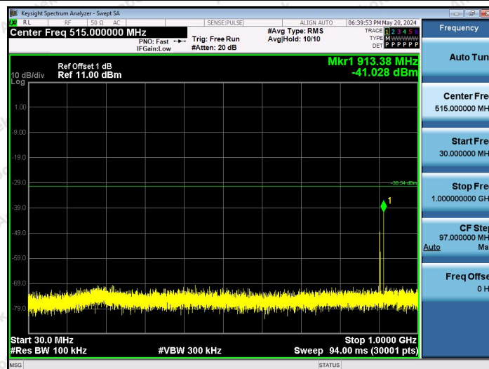
Zigbee-Ant1-2480-30~1000-PASS
