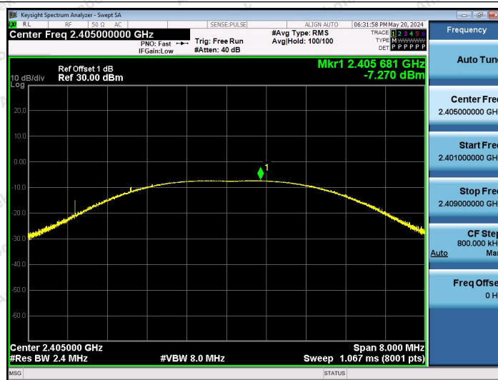
Zigbee-Ant1-2405-PASS
