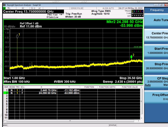
Zigbee-Ant1-2440-1000~26500-PASS
