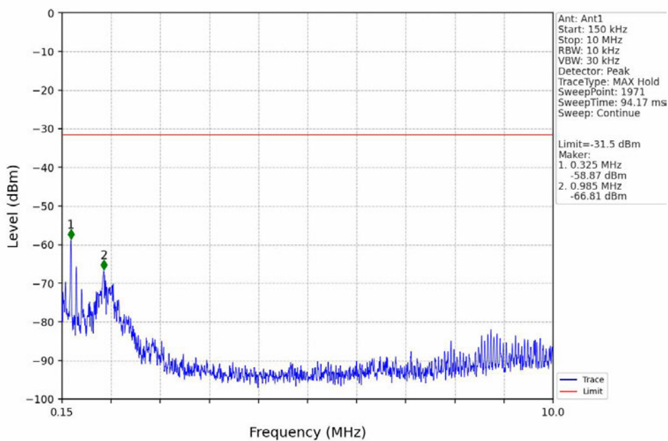
GFSK_DH5_HCH_2480MHz_Ant1_NTNV
