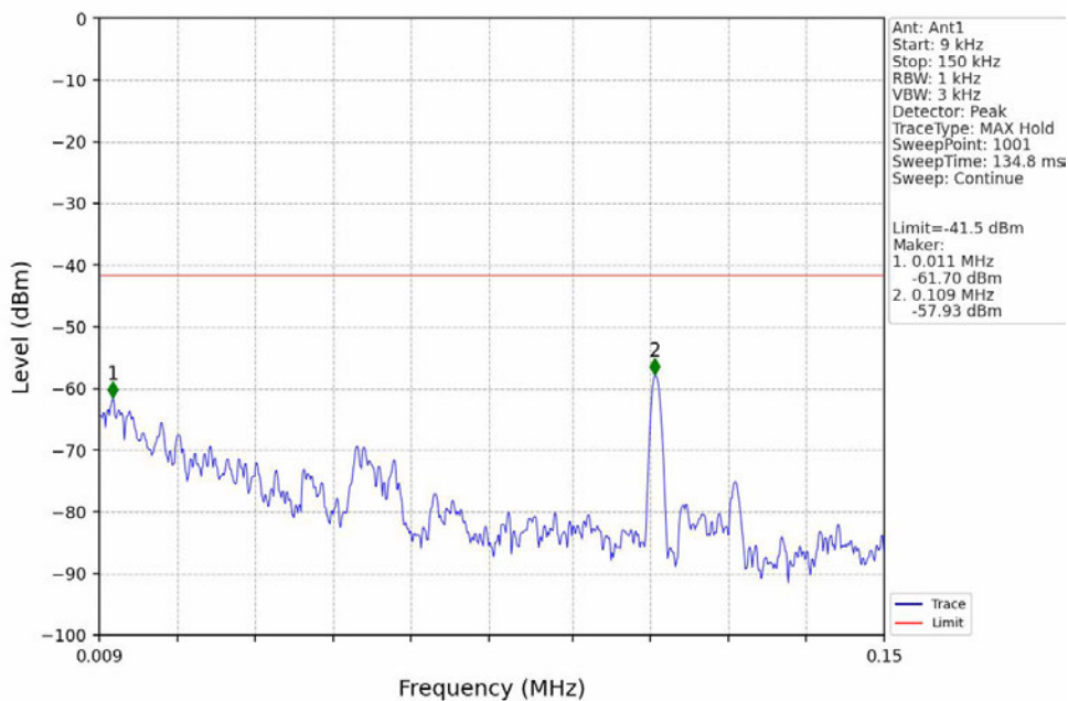
GFSK_DH5_HCH_2480MHz_Ant1_NTNV
