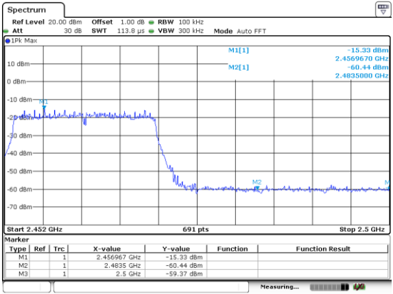
CH11-Bandedge
