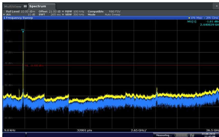
802.11n 20MHz BW Mid Channel
