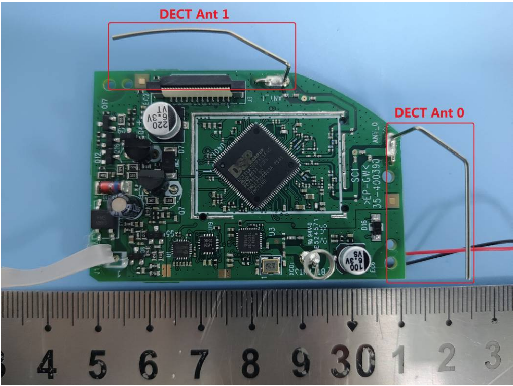
DECT Antenna
