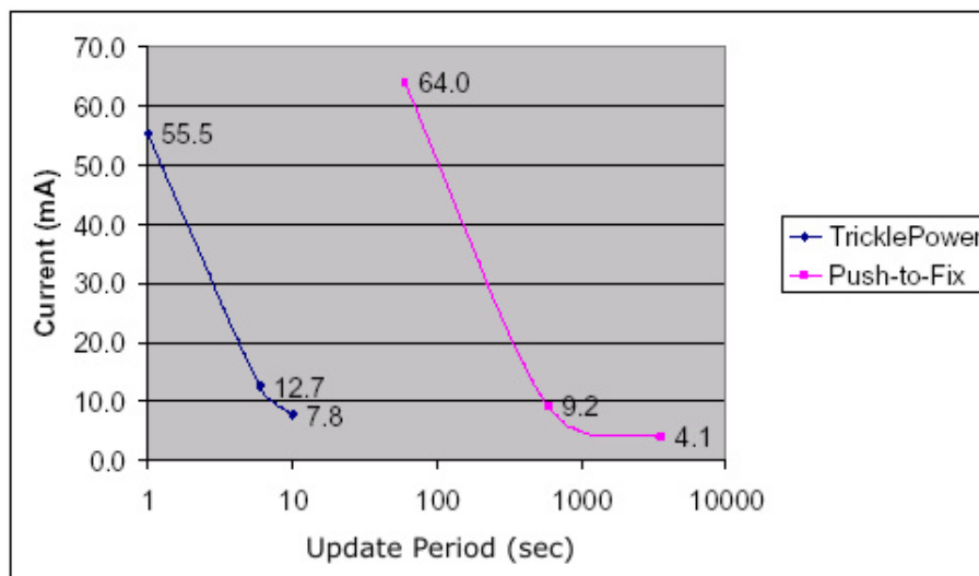
Figure 30: Current comparison between Trickle Power and Push-to Fix mode
