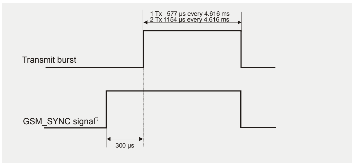
Figure 23: GSM_SYNC signal during transmit burst
