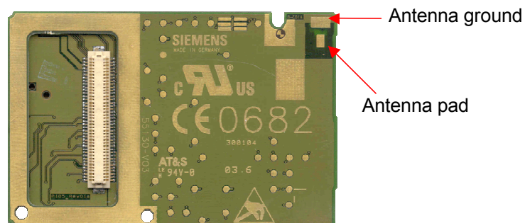
Figure 34: Antenna pad and GND plane
