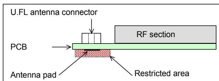
Figure 36: Restricted area around antenna pad
