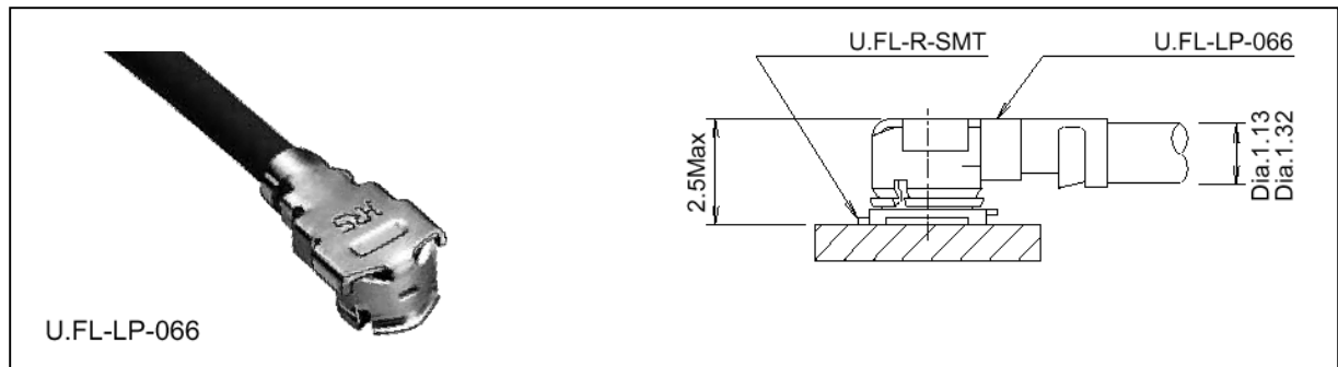
Figure 40: U.FL-R-SMT connector with U.FL-LP-066 plug
