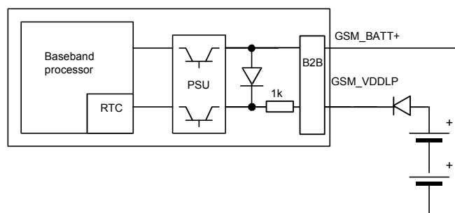
Figure 16: RTC supply from non-chargeable battery
