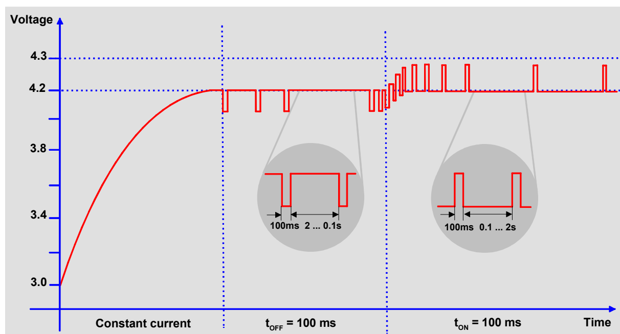
Figure 11: Charging process
