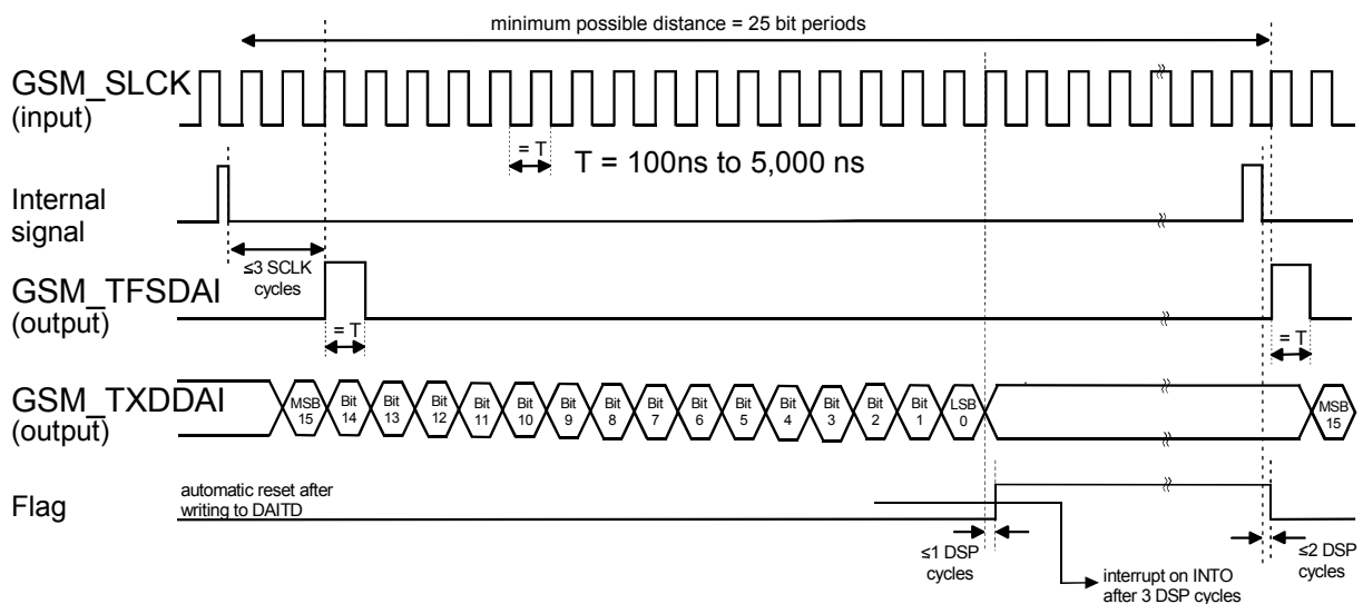
Figure 20: DAI timing on receive path
