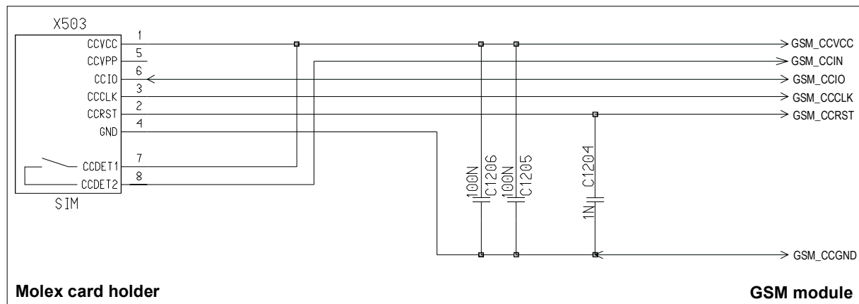
Figure 21: SIM card holder of DSB45 Support Box
