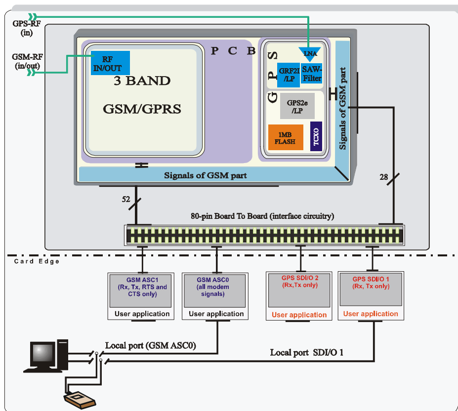
Figure 2: Block diagram of XT55 for SiRF Demo application
