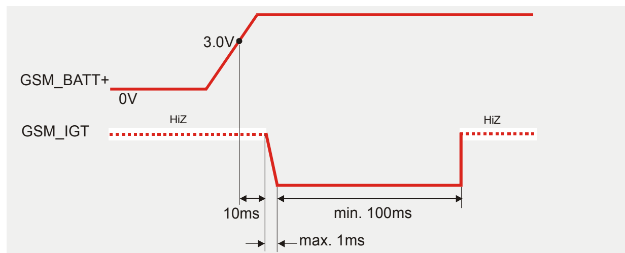
Figure 7: Timing of power-on process if GSM_VDDLPP is fed from external source
