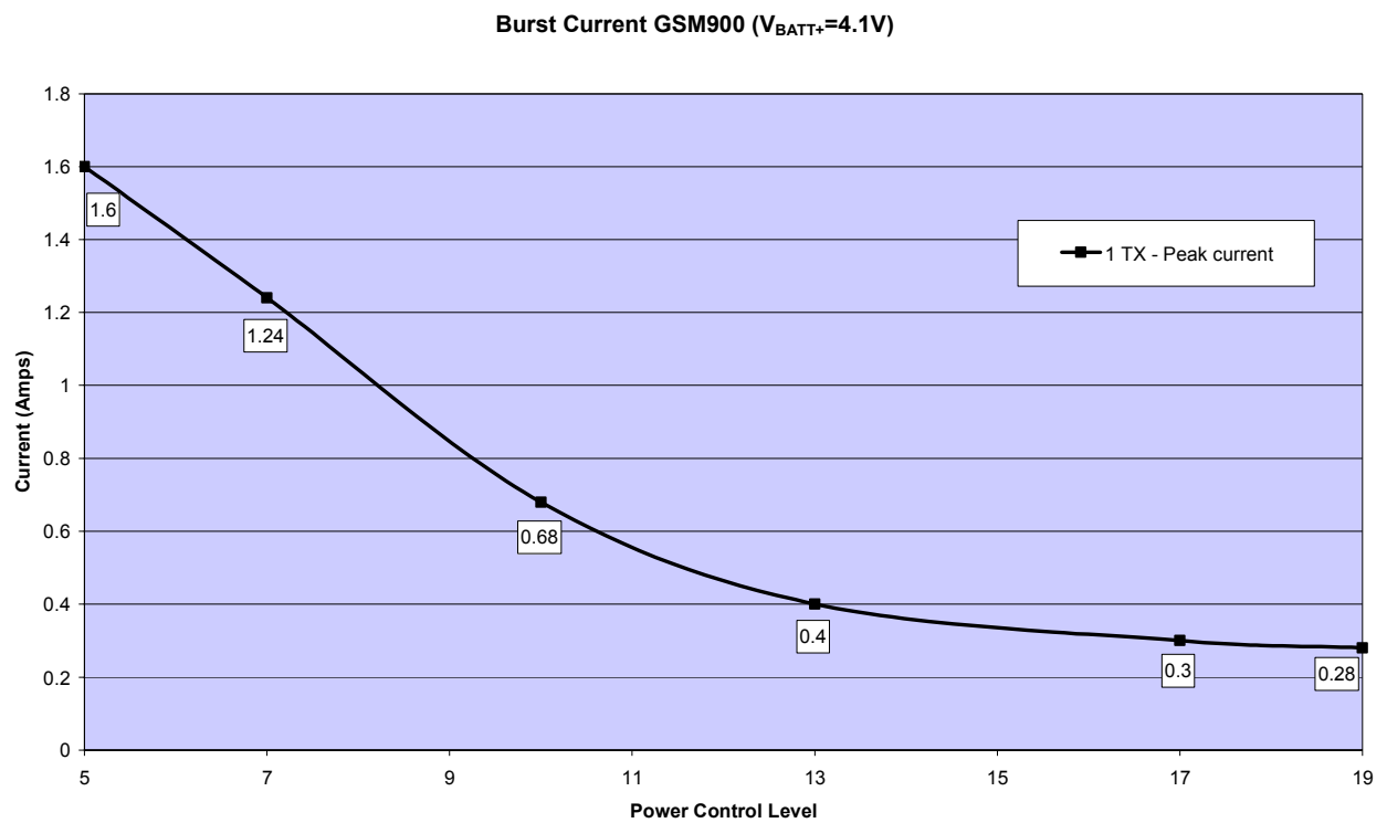
Figure 46: Peak current consumption during transmit burst in EGSM 900 network
