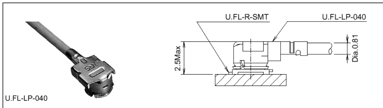
Figure 39: U.FL-R-SMT connector with U.FL-LP-040 plug
