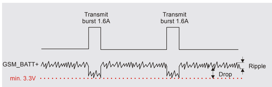
Figure 4: Power supply limits during transmit burst
