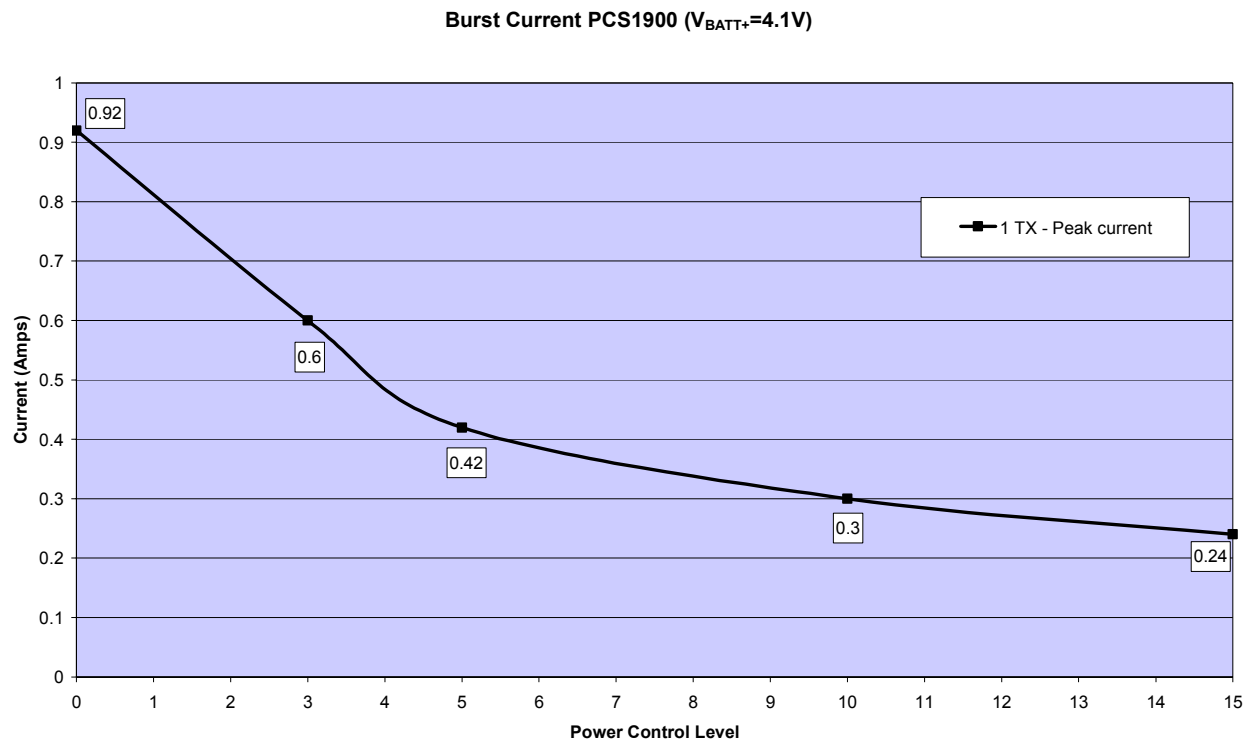
Figure 48: Peak current consumption during transmit burst in GSM 1900 network
