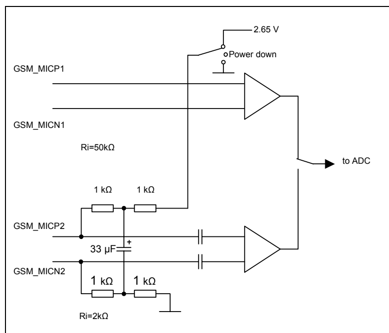
Figure 18: Schematic of microphone inputs
