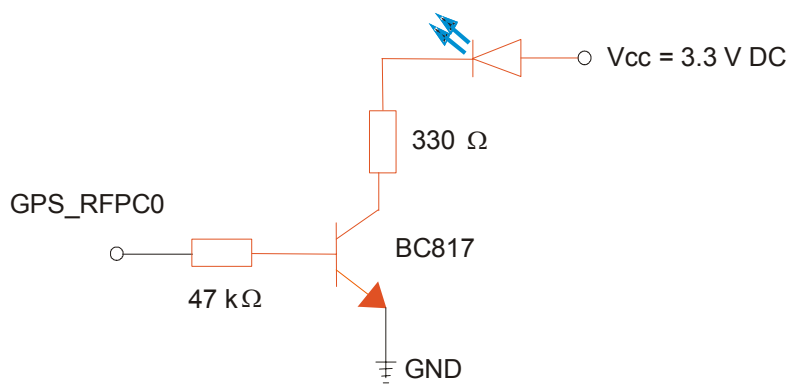
Figure 31: Example of LED circuit
