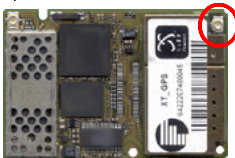
Figure 37: GPS antenna connector (U.FL-R-SMT connector)
