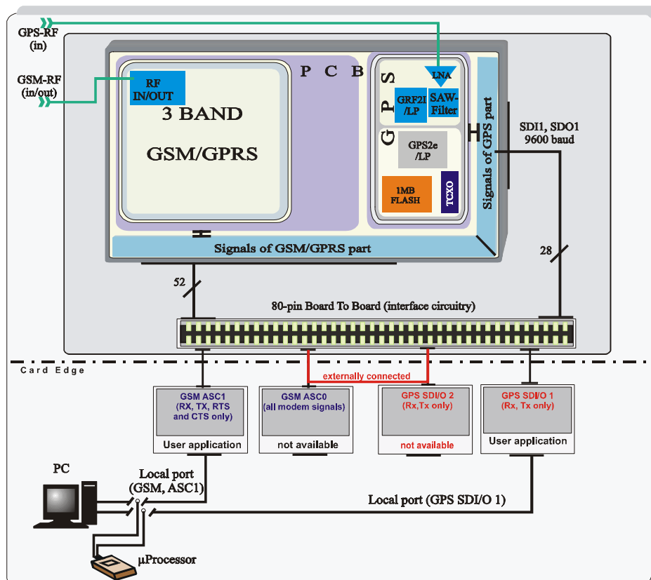
Figure 3: Block diagram of XT55 with AVL or TCP/IP application (optional)
