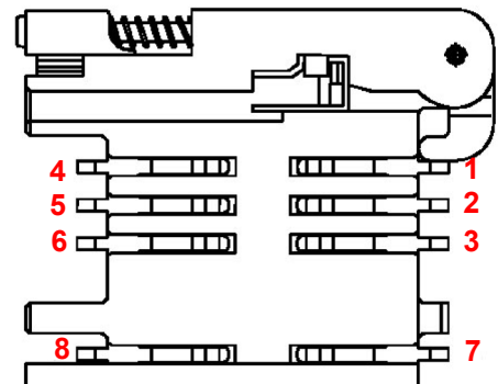
Figure 22: Pin numbers of Molex SIM card holder on DSB45 Support Box
