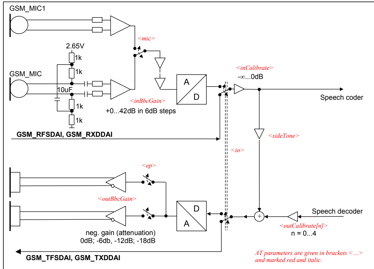
Figure 50: AT audio programming model
