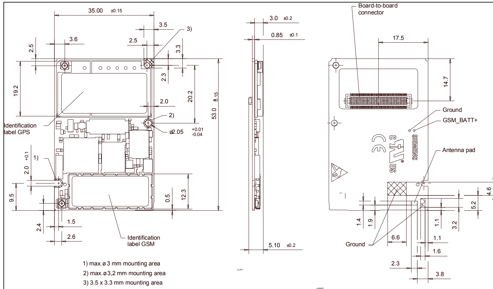
Figure 53: Mechanical dimensions of XT55
