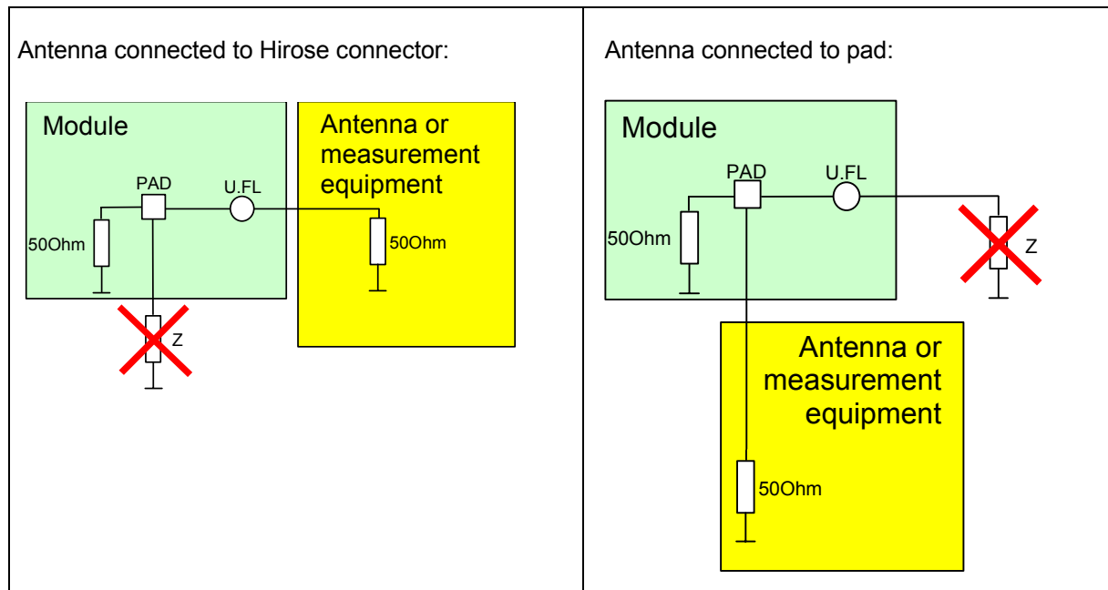
Figure 35: Never use antenna connector and antenna pad at the same time
