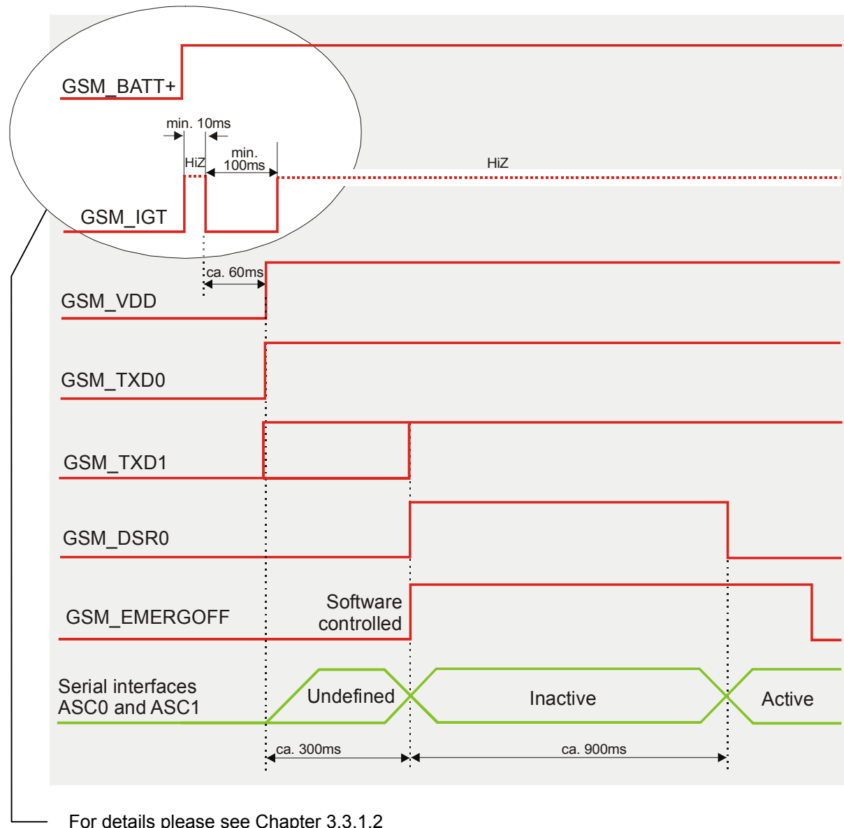
Figure 5: Power-on by ignition signal
