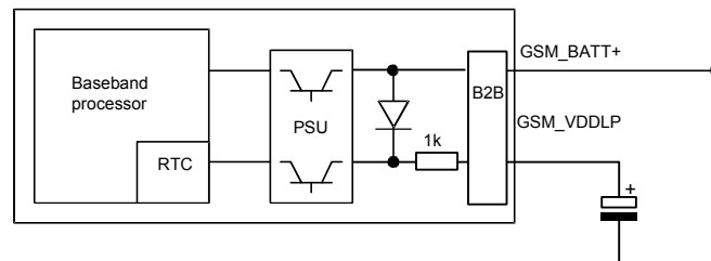
Figure 14: RTC supply from capacitor
