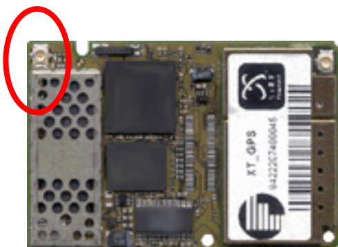
Figure 33: U.FL-R-SMT connector
