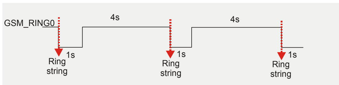
Figure 25: Incoming voice call
