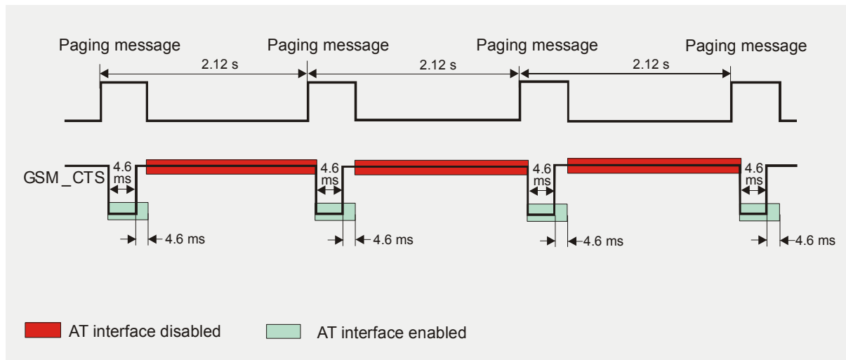
Figure 12: Timing of CTS signal (example for a 2.12 s paging cycle)
