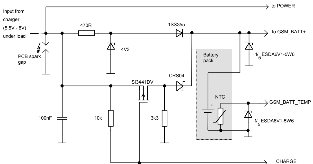
Figure 9: Schematic of approved charging transistor, trickle charging and ESD protection
