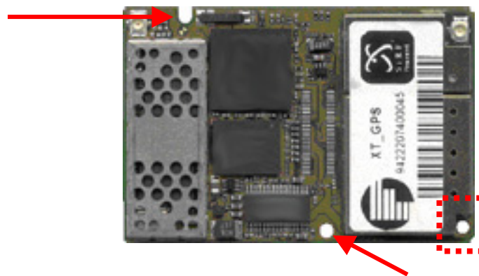
Figure 54: Mounting holes on XT55
