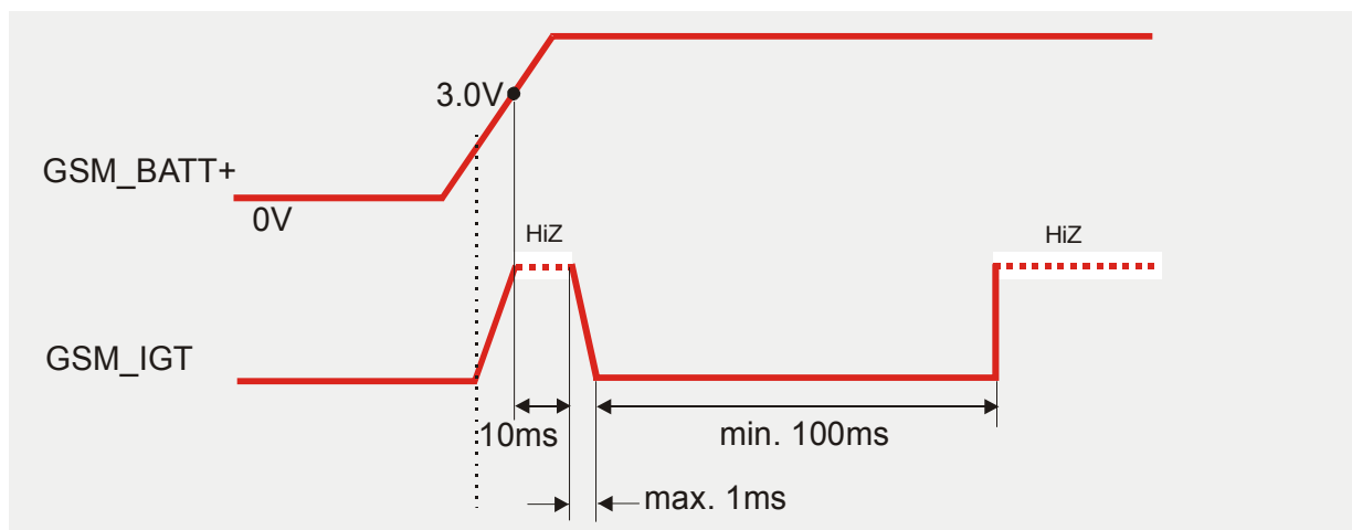
Figure 6: Timing of power-on process if GSM_VDDLPP is not used
