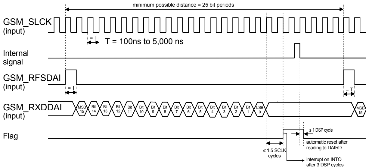
Figure 19: DAI timing on transmit path
