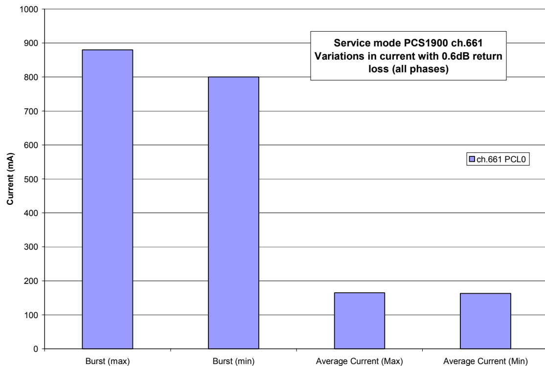
Figure 49: Typical current consumption vs. return loss
