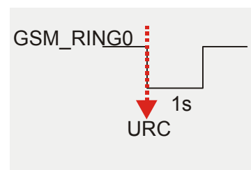
Figure 27: URC transmission
