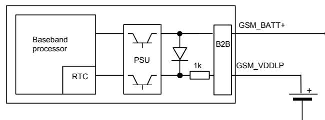
Figure 15: RTC supply from rechargeable battery
