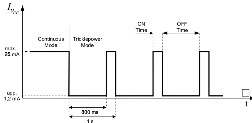
Figure 29: Example for current in Trickle Power mode
