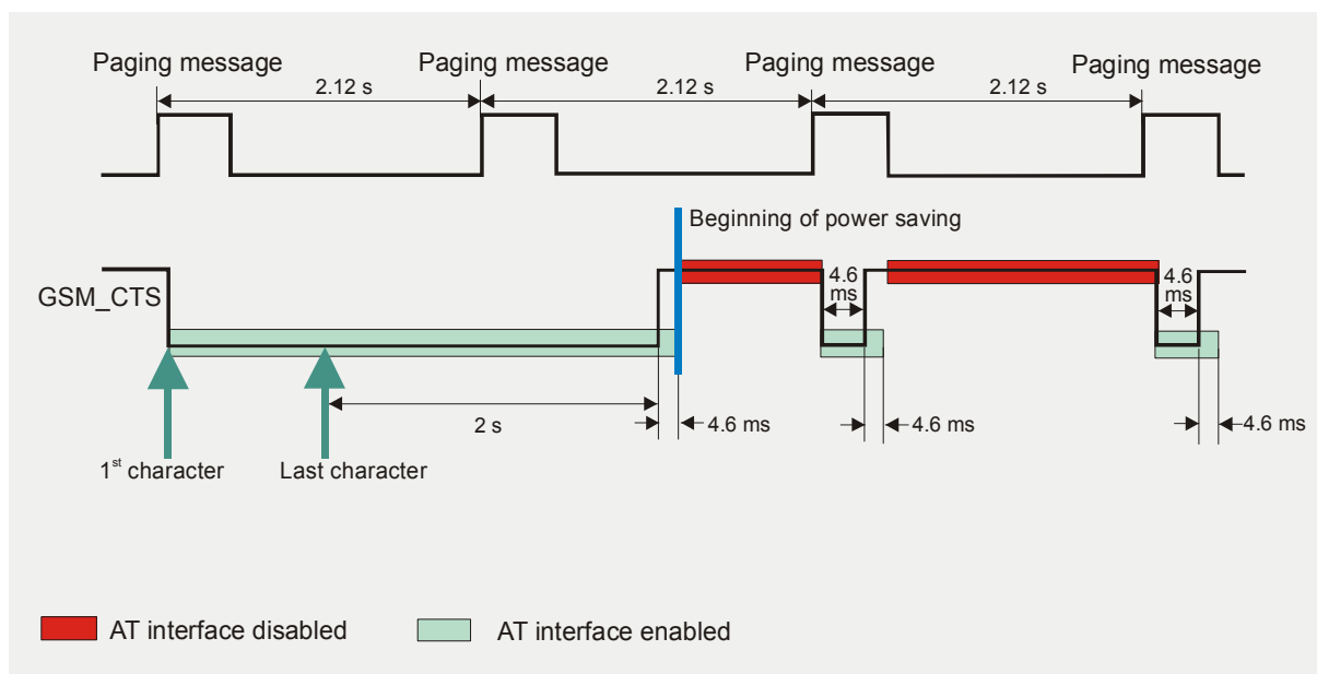
Figure 13: Beginning of power saving if CFUN=5 or 7
