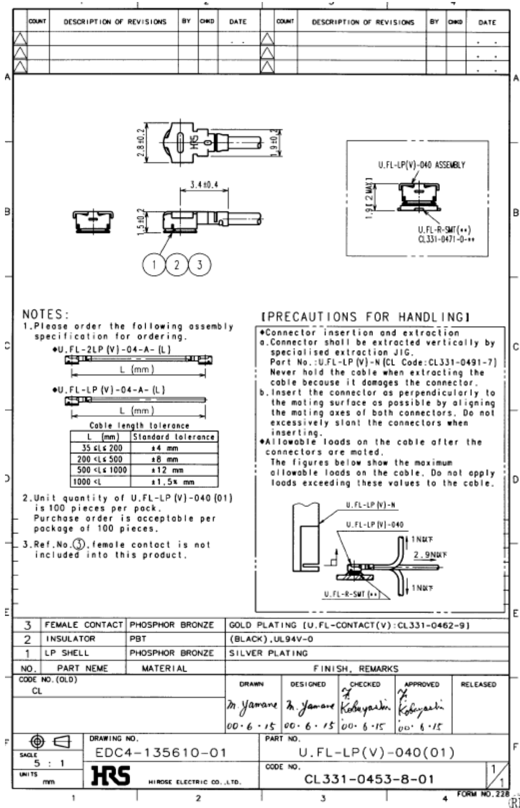
Figure 41: Specifications of U.FL-LP-(V)-040(01) plug
