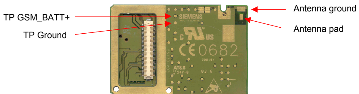
Figure 52: XT55 bottom view
