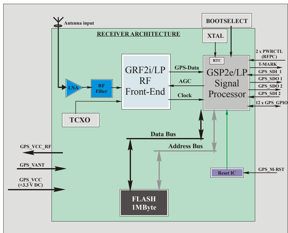
Figure 32: Receiver architecture of the GPS receiver
