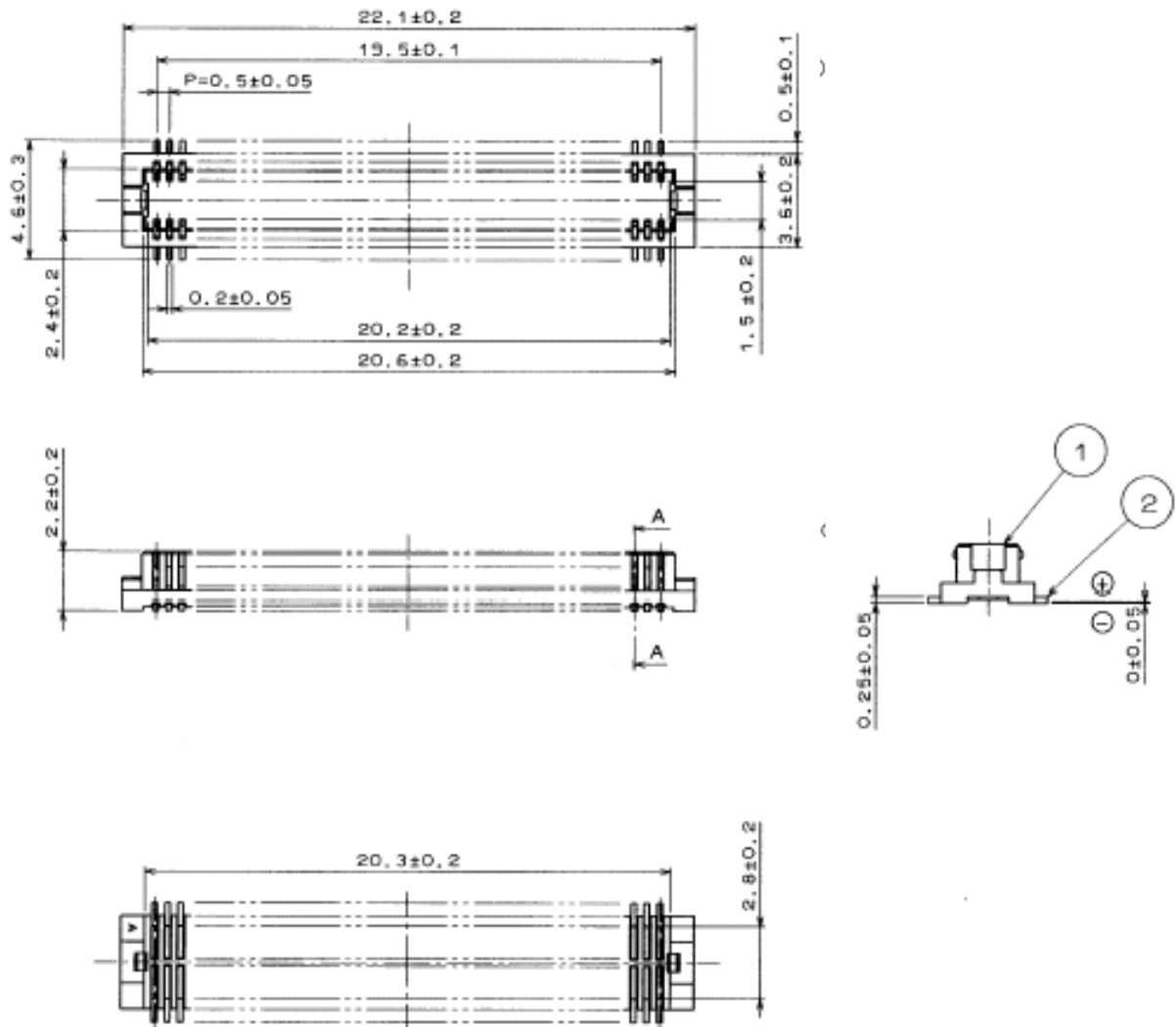
Figure 56: Mechanical dimensions of Hirose DF12 connector
