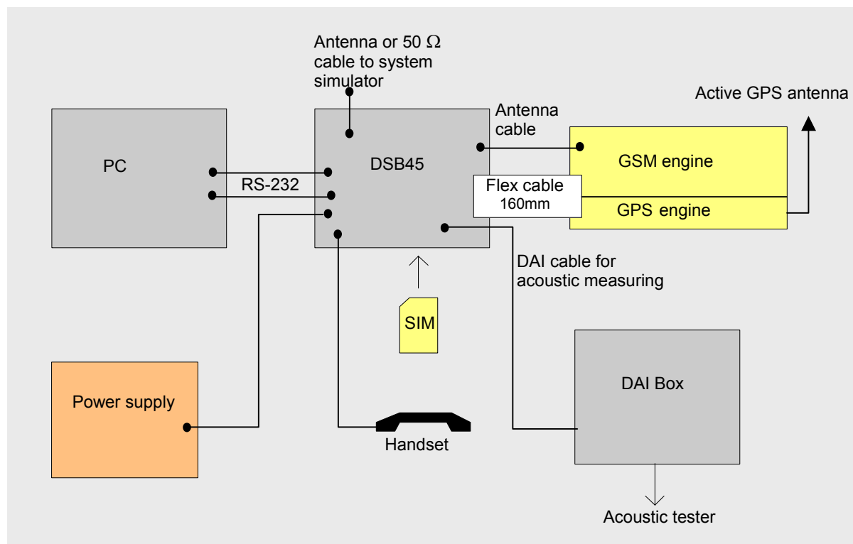
Figure 57: Reference equipment for approval
