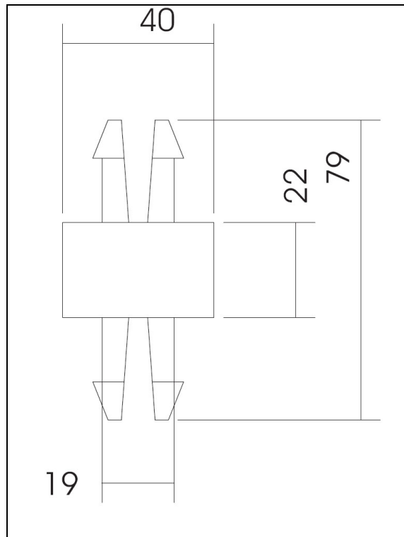
Figure 55: Recommended dowel
