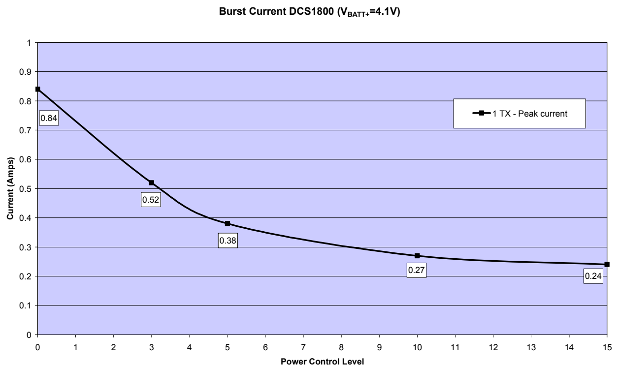
Figure 47: Peak current consumption during transmit burst in GSM 1800 network
