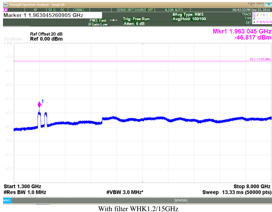
Plot 3.5.7: Spurious Emission Conducted Measurement, AWGN 4.1MHz, Fc = 751.5 MHz, 1.3 GHz – 8 GHz
