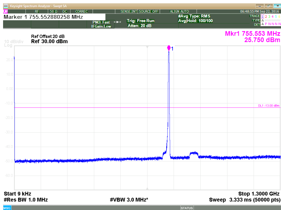
Plot 3.5.11: Spurious Emission Conducted Measurement, AWGN 4.1MHz, Fc = 754.5 MHz, 9 kHz – 1.3 GHz
