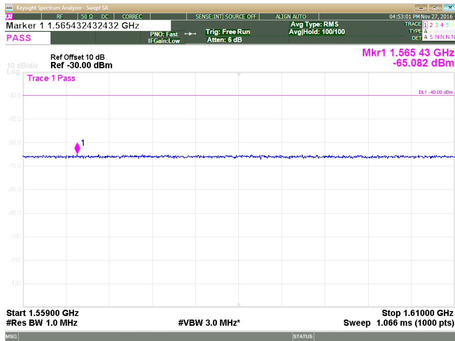
Plot 3.5.10: Spurious Emission Conducted Measurement, AWGN 4.1MHz, Fc = 751.5 MHz, 1559 MHz – 1610 MHz
