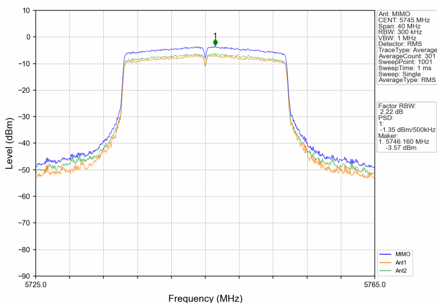
802.11ax(HEW20)_LCH_5745MHz_RU242_Left_MIMO_NTNV
