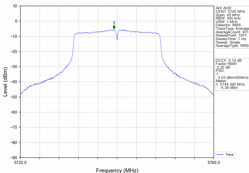
802.11n(HT20)_LCH_5745MHz_Ant2_NTNV
