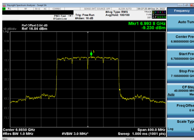
Plot 7-336. Power Spectral Density Plot SDM Antenna WF5b (160MHz 802.11ax (UNII Band 8) – Ch. 207, MCS11)
