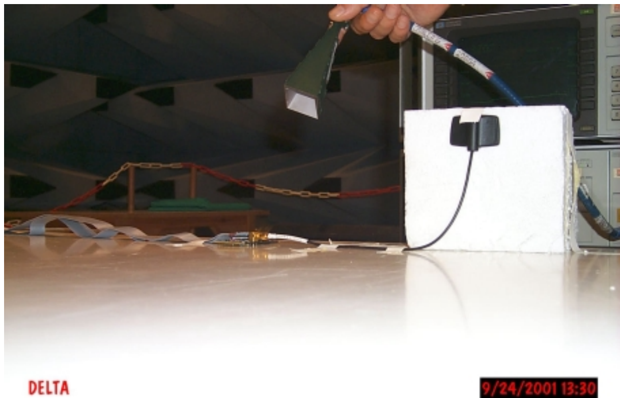
PHOTO A2.5 Test set-up for test 18-26 GHz
