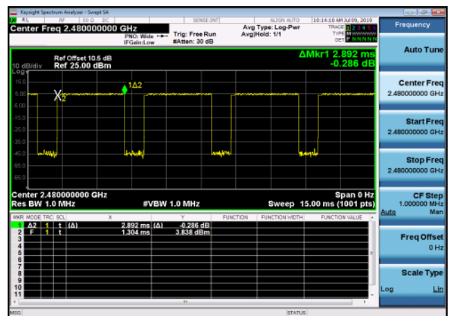
8PSK,2480,3DH5,Transmission Time
