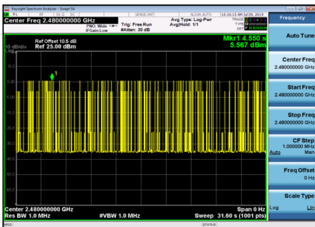
8PSK,2480,3DH5,Transmission Number
