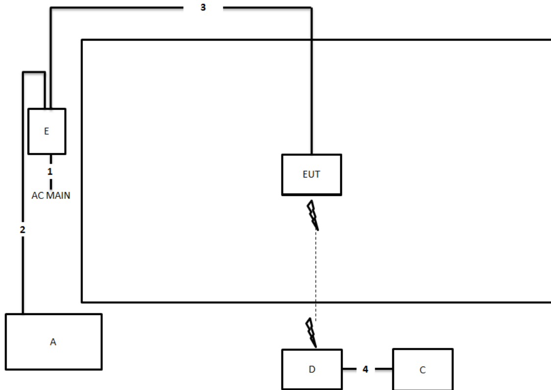
Test Setup Diagram - Radiated Test > 1GHz, Beamforming Mode
