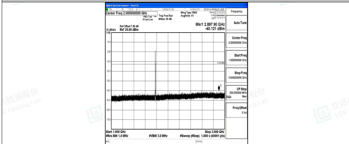
Band66_3MHz_QPSK_132657_1RB#0_1000~3000_1000~3000
