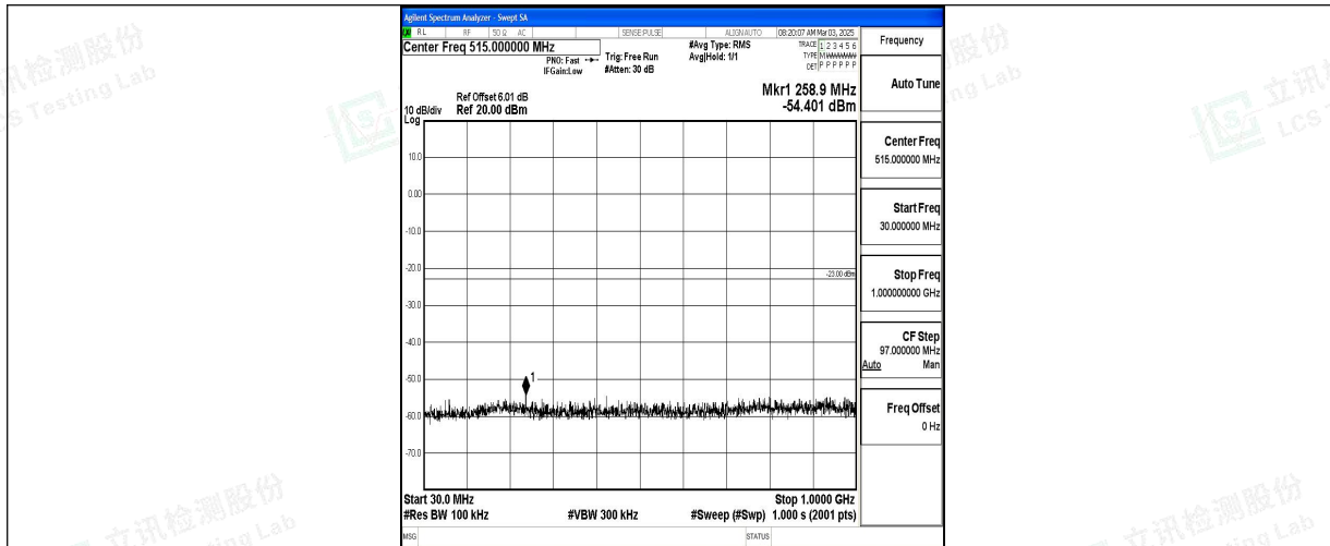
Band66_3MHz_QPSK_132657_1RB#0_30~1000_30~1000
