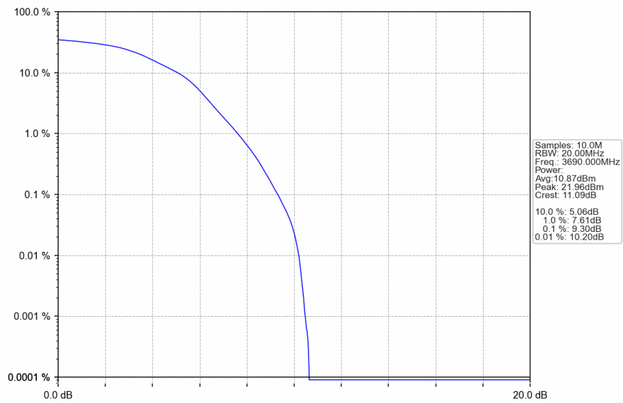
n48_30kHz_SISO_NTNV_20MHz_DFT-s-OFDM_16_QAM_3690MHz_Outer_Full
