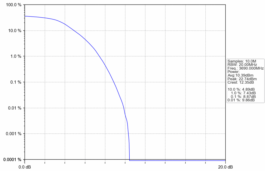
n48_30kHz_SISO_NTNV_20MHz_DFT-s-OFDM_QPSK_3690MHz_Outer_Full
