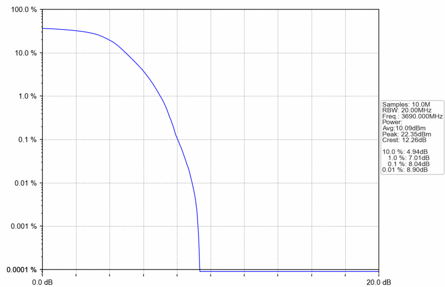
n48_30kHz_SISO_NTNV_20MHz_DFT-s-OFDM_PI/2_BPSK_3690MHz_Outer_Full
