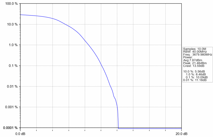
n48_30kHz_SISO_NTNV_40MHz_DFT-s-OFDM_16_QAM_3679.98MHz_Outer_Full
