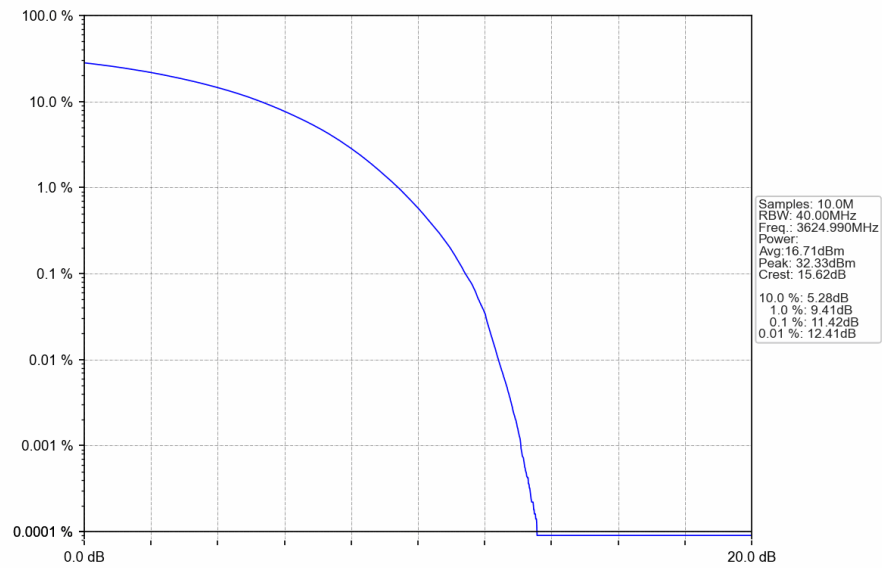
n48_30kHz_SISO_NTNV_40MHz_CP-OFDM_256_QAM_3624.99MHz_Outer_Full
