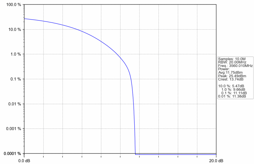
n48_30kHz_SISO_NTNV_20MHz_CP-OFDM_QPSK_3560.01MHz_Outer_Full
