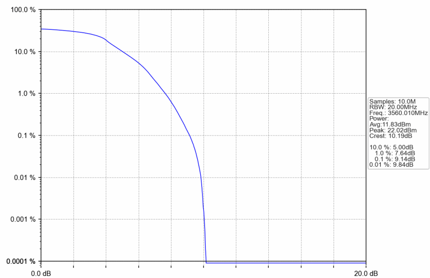
n48_30kHz_SISO_NTNV_20MHz_DFT-s-OFDM_QPSK_3560.01MHz_Outer_Full
