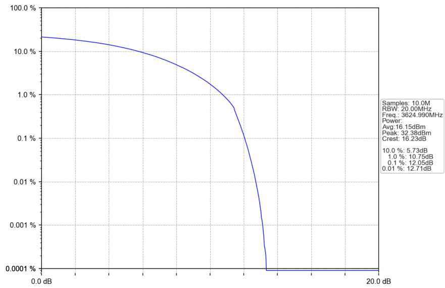
n48_30kHz_SISO_NTNV_20MHz_CP-OFDM_16_QAM_3624.99MHz_Outer_Full
