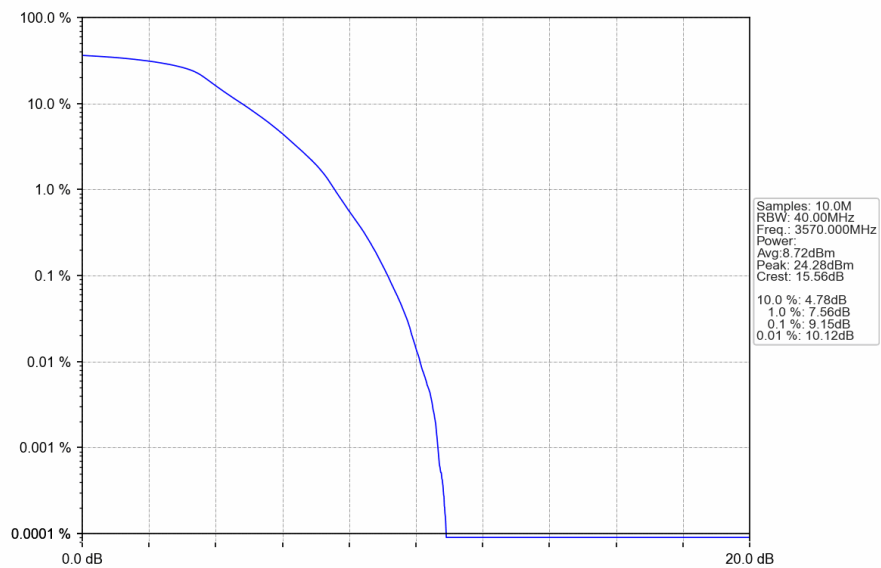
n48_30kHz_SISO_NTNV_40MHz_DFT-s-OFDM QPSK_3570MHz_Outer_Full
