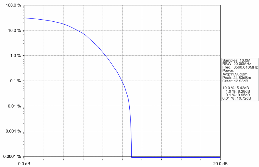
n48_30kHz_SISO_NTNV_20MHz_DFT-s-OFDM_64_QAM_3560.01MHz_Outer_Full
