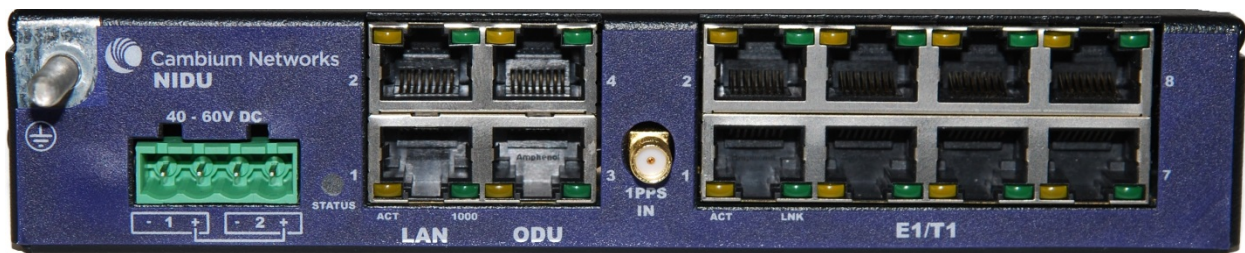
Figure 34 NIDU interfaces
