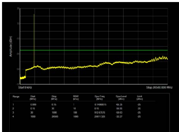
LTE Band 7 15MHz CH- Middle 9kHz~26.5GHz
