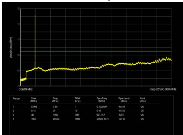
LTE Band 7 15MHz CH-High 9kHz~26.5GHz
