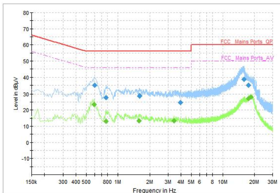
Fig.49 AC Power line Conducted Emission (Traffic, 120V), 1M
