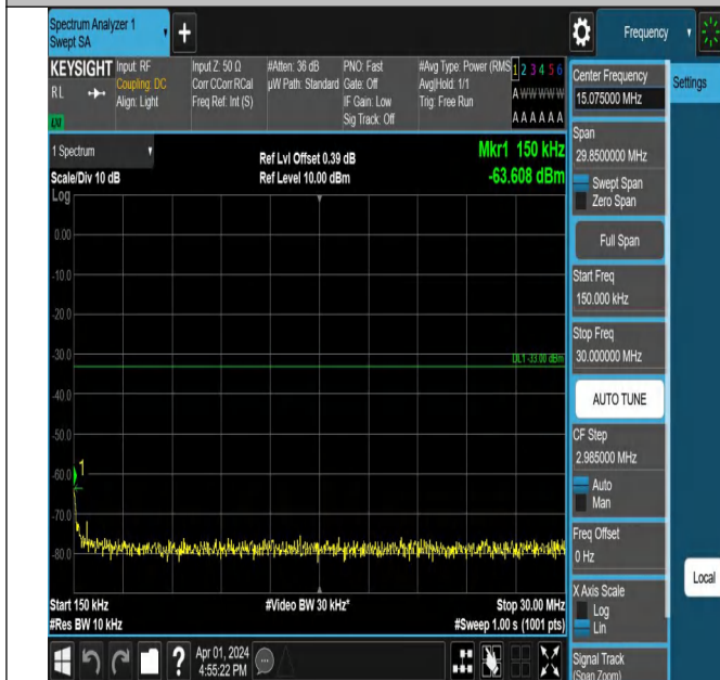
Band4-1413-3-0.15~30MHz-PASS
