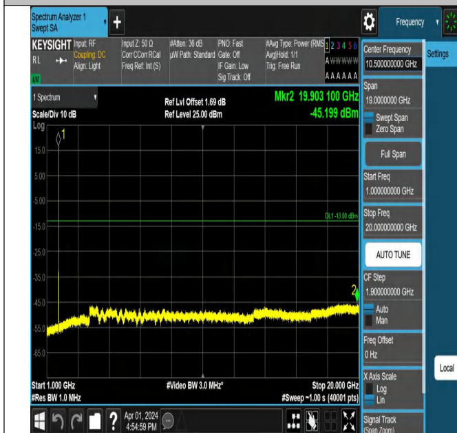
Band4-1312-3-1000~20000MHz-PASS
