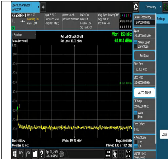
Band4-1413-1-0.15~30MHz-PASS
