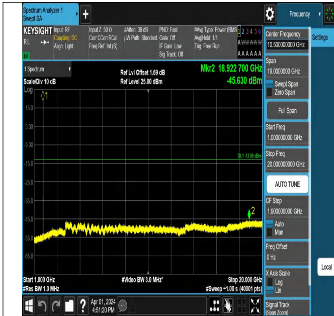
Band4-1413-1-1000~20000MHz-PASS
