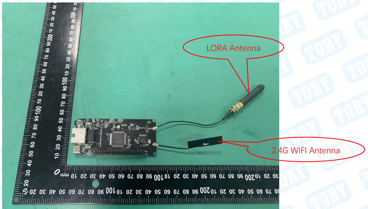
Photo 2 Appearance of PCB
