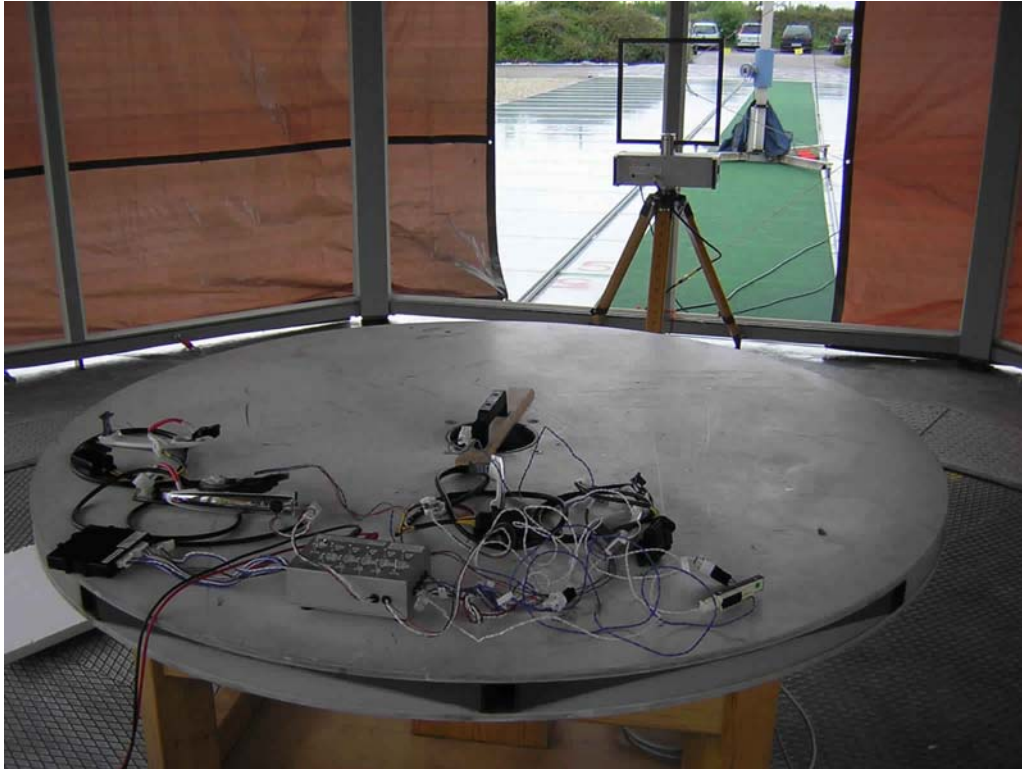
Trunk Antenna
