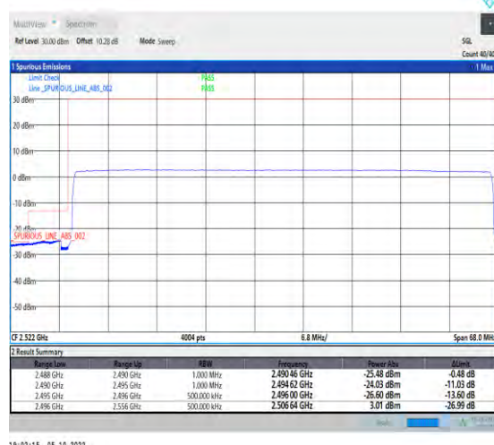
1-N41-PC2-30-60-L-6-CP-QPSK-Outer_Full-162 @0-Ant1-1--PASS-see graph
