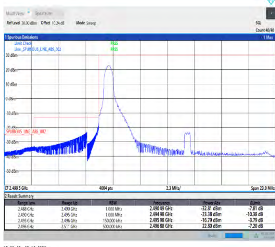
1-N41-PC2-30-15-L-4-CP-QPSK-Edge_1RB_Left-1@0 -Ant1-1--PASS-see graph
