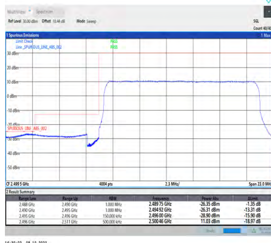
1-N41-PC2-30-15-L-3-DFT-QPSK-Outer_Full-36@ 0-Ant1-1--PASS-see graph
