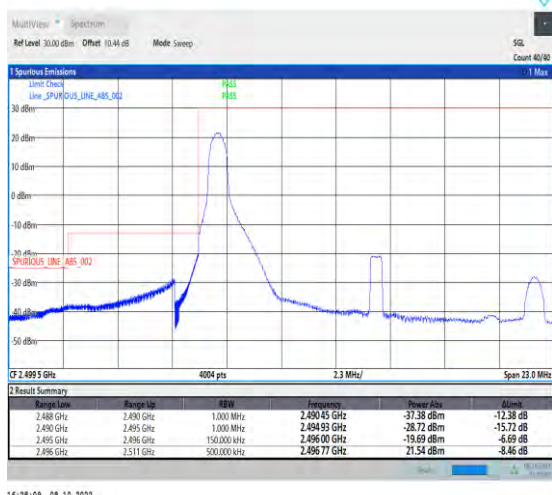
1-N41-PC2-30-15-L-1-DFT-QPSK-Edge_1RB_Left-1@ 0-Ant1-1--PASS-see graph
