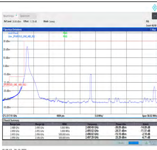
1-N41-PC2-30-50-L-1-DFT-PI2BPSK-Edge_1RB_Left-1@0-Ant1-1--PASS-see graph
