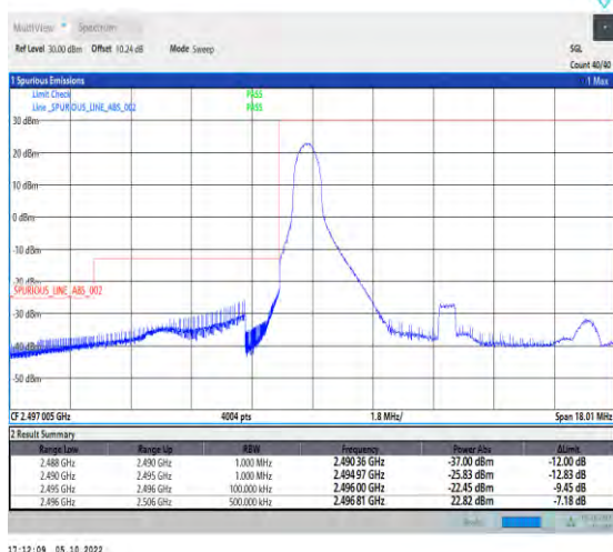
1-N41-PC2-30-10-L-1-DFT-QPSK-Edge_1RB_Left-1@ 0-Ant1-1--PASS-see graph
