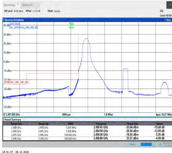
1-N41-PC2-30-10-L-1-DFT-PI2BPSK-Edge_1RB_Left-1@0-Ant1-1--PASS-see graph
