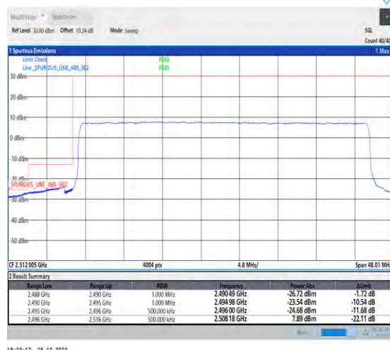
1-N41-PC2-30-40-L-3-DFT-QPSK-Outer_Full-100 @0-Ant1-1--PASS-see graph
