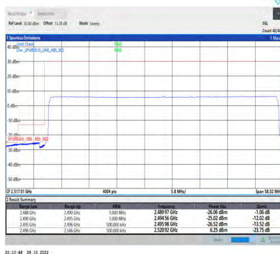
1-N41-PC2-30-50-L-6-CP-QPSK-Outer_Full-133@0-Ant1-1--PASS-see graph
