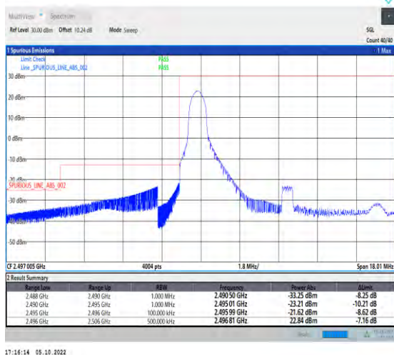
1-N41-PC2-30-10-L-4-CP-QPSK-Edge_1RB_Left-1@0 -Ant1-1--PASS-see graph
