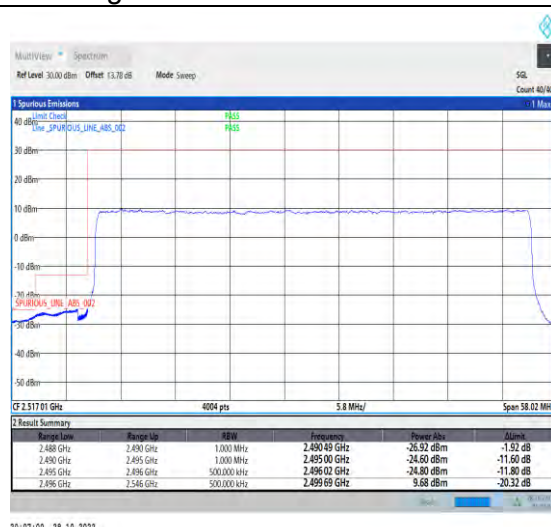
1-N41-PC2-30-50-L-3-DFT-PI2BPSK-Outer_Full-128@0-Ant1-1--PASS-see graph
