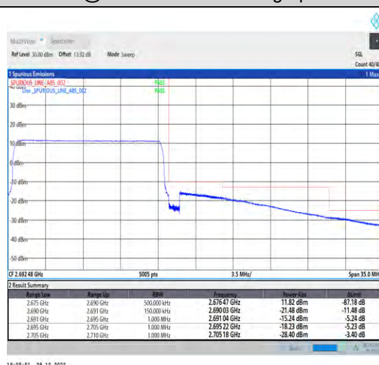
1-N41-PC2-30-15-H-6-CP-QPSK-Outer_Full-38@ 0-Ant1-1--PASS-see graph
