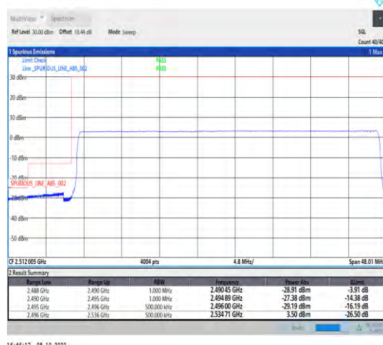
1-N41-PC2-30-40-L-6-CP-QPSK-Outer_Full-106 @0-Ant1-1--PASS-see graph
