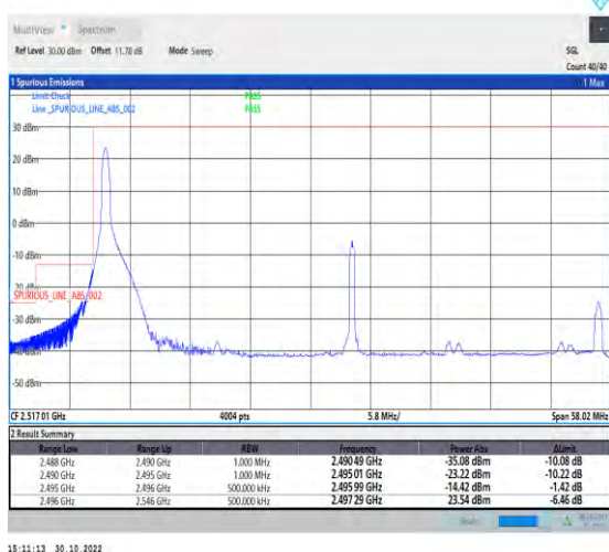
1-N41-PC2-30-50-L-4-CP-QPSK-Edge_1RB_Left-1@0-Ant1-1--PASS-see graph
