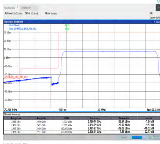
1-N41-PC2-30-15-L-6-CP-QPSK-Outer_Full-38@ 0-Ant1-1--PASS-see graph
