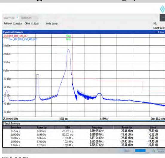
1-N41-PC2-30-15-H-5-CP-QPSK-Edge_1RB_Right-1 @37-Ant1-1--PASS-see graph
