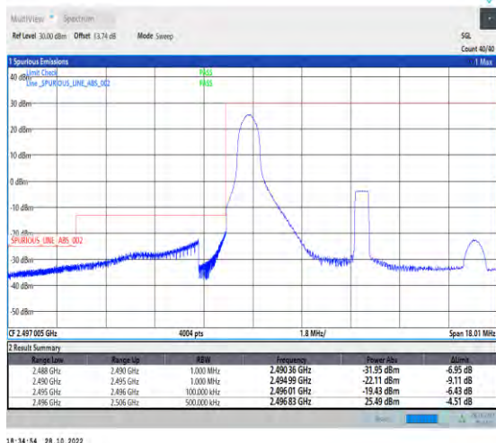
1-N41-PC2-30-10-L-4-CP-QPSK-Edge_1RB_Left-1@0-Ant1-1--PASS-see graph
