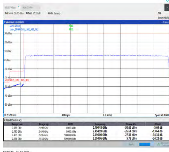
1-N41-PC2-30-60-L-3-DFT-QPSK-Outer_Full-162 @0-Ant1-1--PASS-see graph
