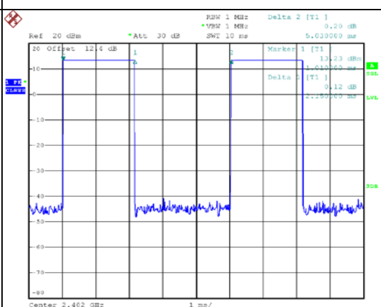
BLE_1 Mbps
