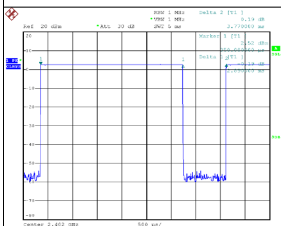
BT_1 Mbps
