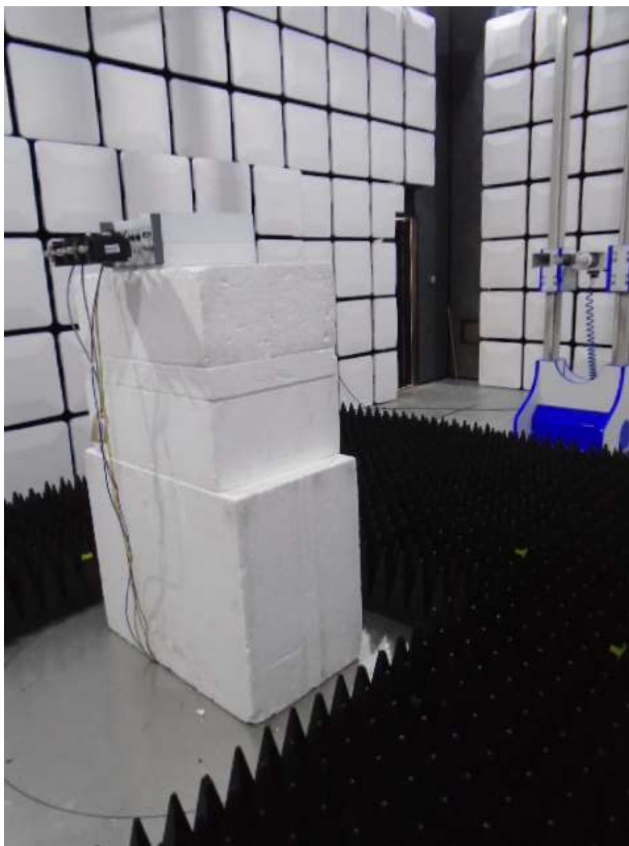
Radiated 8GHz – 18GHz Testing
