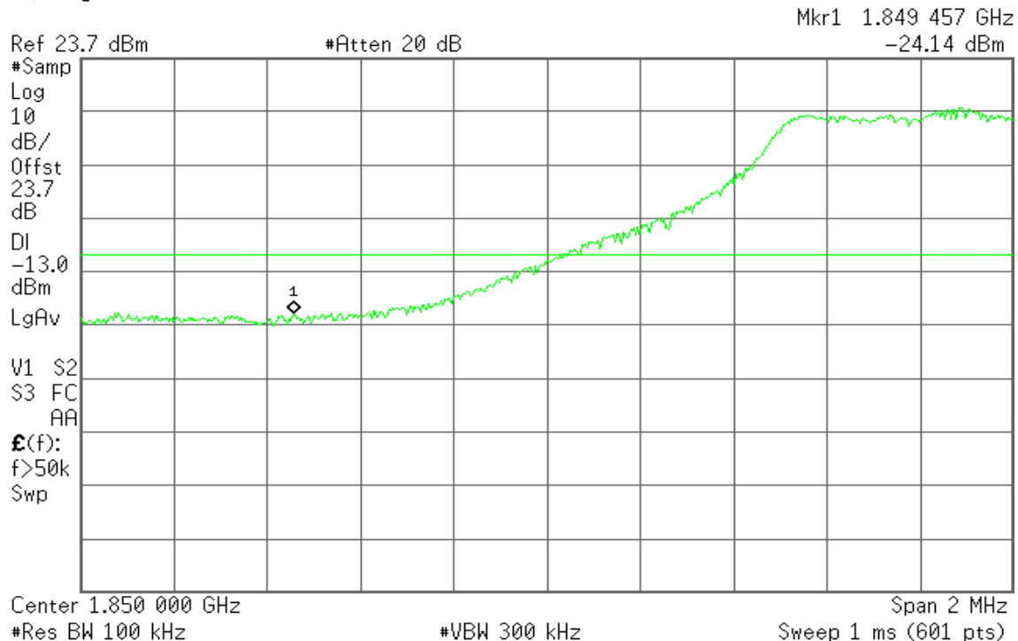
Figure 16-1: Band Edge emissions – CH Low
