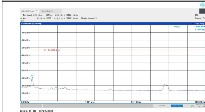
Band5-4132-4-0.009~0.15MHz-PASS
