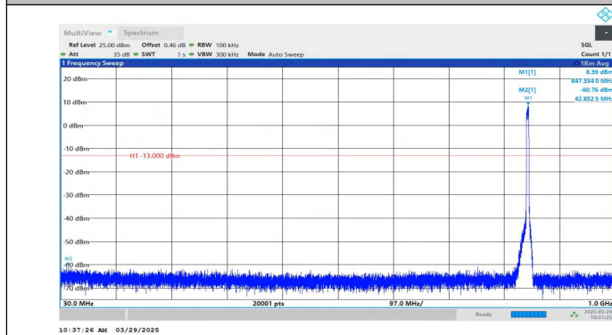
Band5-4233-3-30~1000MHz-PASS
