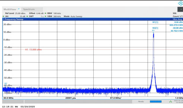
Band5-4182-2-30~1000MHz-PASS
