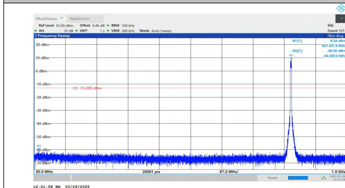
Band5-4132-4-30~1000MHz-PASS
