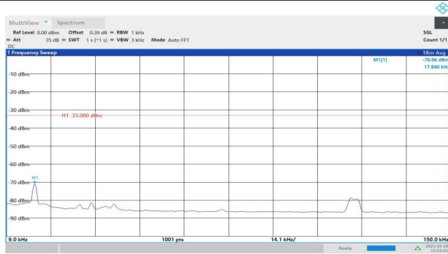
Band5-4233-4-0.009~0.15MHz-PASS
