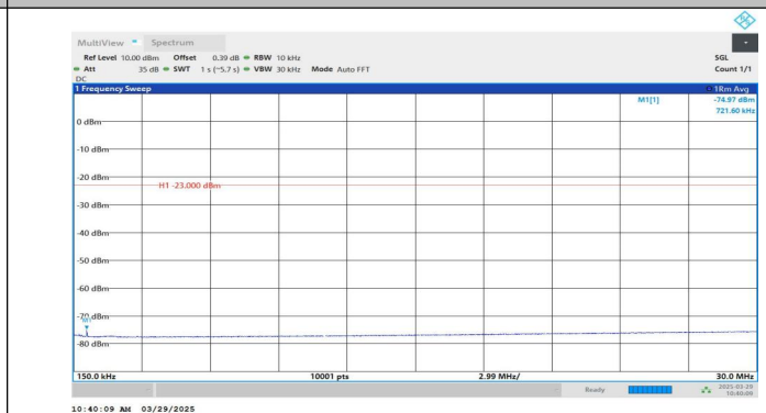
Band5-4233-4-0.15~30MHz-PASS
