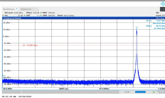
Band5-4132-30~1000MHz-PASS
