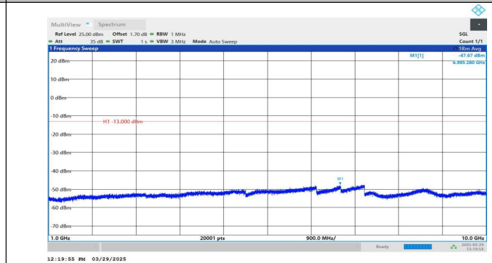
Band5-4132-3-1000~10000MHz-PASS
