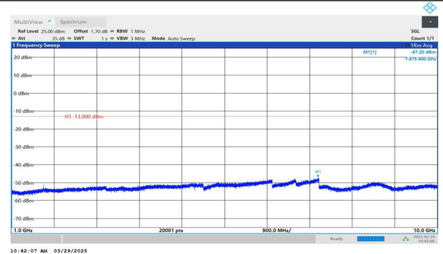
Band5-4182-5-1000~10000MHz-PASS
