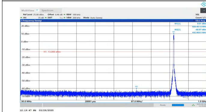
Band5-4132-3-30~1000MHz-PASS
