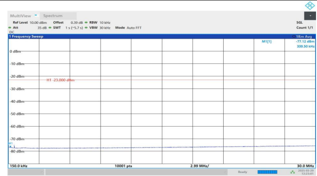
Band5-4233-4-0.15~30MHz-PASS
