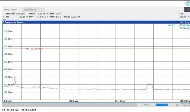
Band5-4132-0.009~0.15MHz-PASS
