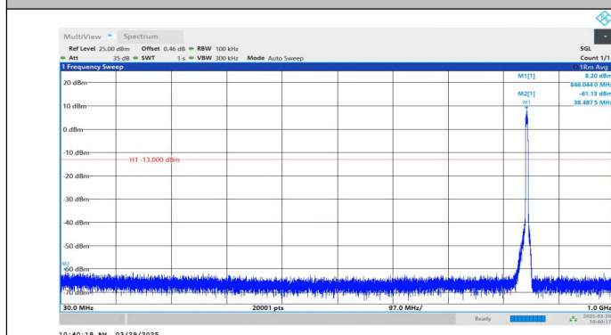
Band5-4233-4-30~1000MHz-PASS
