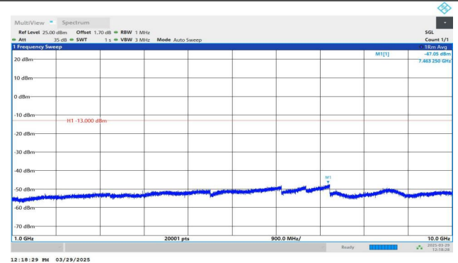
Band5-4182-2-1000~10000MHz-PASS
