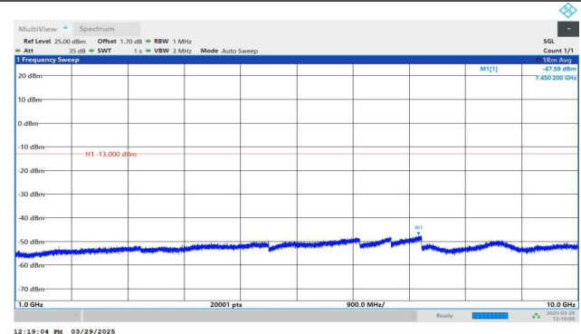
Band5-4233-2-1000~10000MHz-PASS
