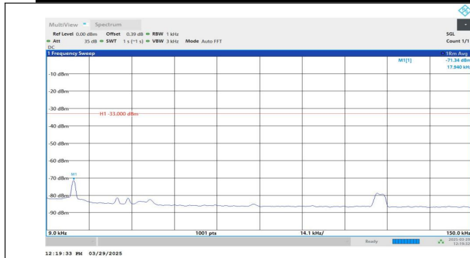
Band5-4132-3-0.009~0.15MHz-PASS
