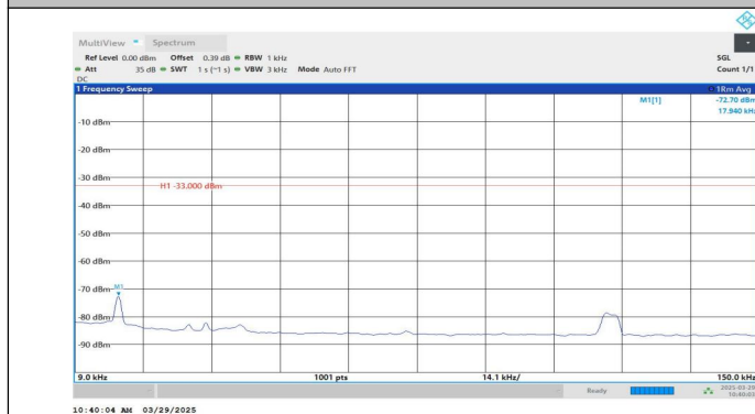
Band5-4233-4-0.009~0.15MHz-PASS
