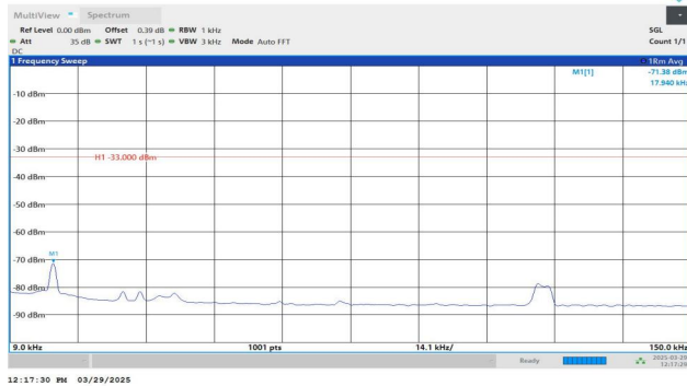
Band5-4132-2-0.009~0.15MHz-PASS
