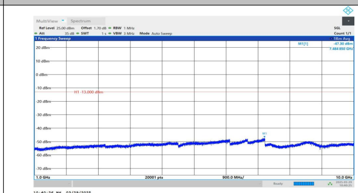
Band5-4233-4-1000~10000MHz-PASS
