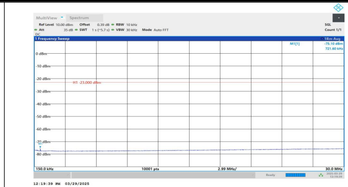
Band5-4132-3-0.15~30MHz-PASS
