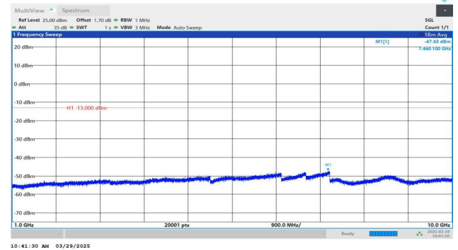
Band5-4132-5-1000~10000MHz-PASS
