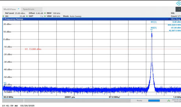
Band5-4182-5-30~1000MHz-PASS
