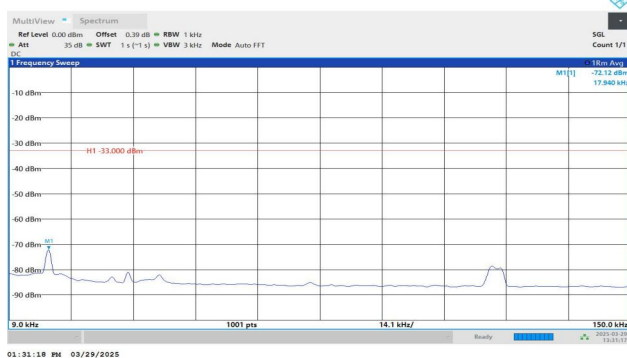
Band5-4182-1-0.009~0.15MHz-PASS
