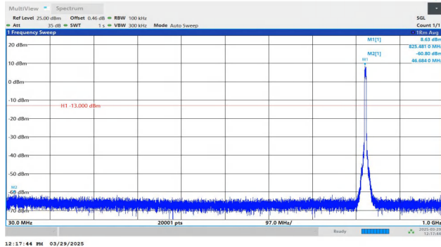
Band5-4132-2-30~1000MHz-PASS
