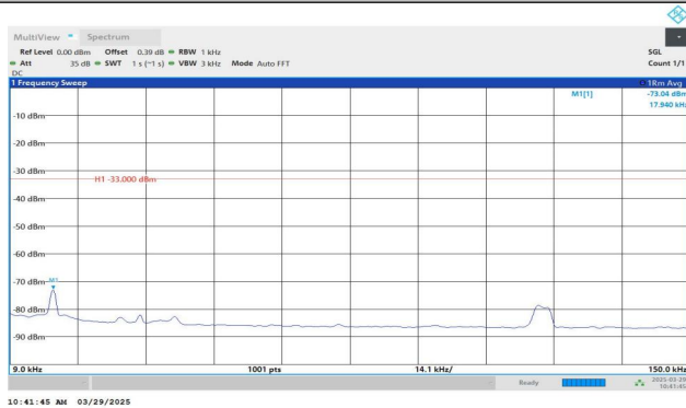
Band5-4182-5-0.009~0.15MHz-PASS
