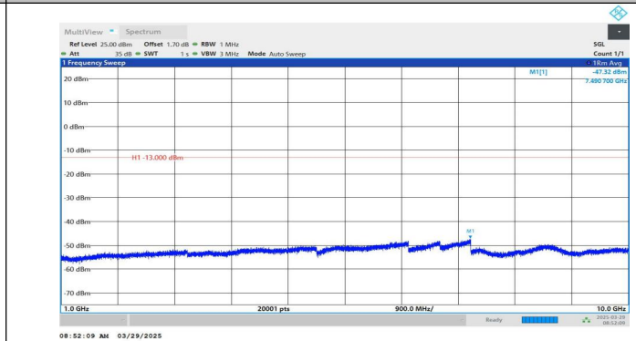
Band5-4233-1000~10000MHz-PASS
