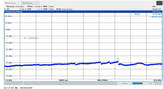
Band5-4132-2-1000~10000MHz-PASS
