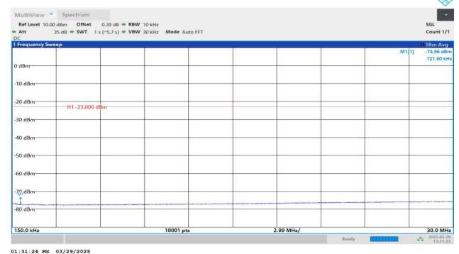
Band5-4182-1-0.15~30MHz-PASS
