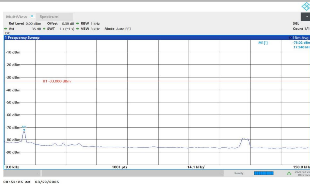
Band5-4182-0.009~0.15MHz-PASS
