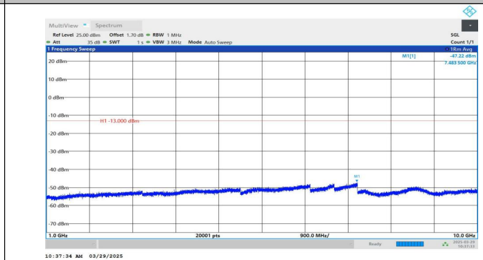
Band5-4233-3-1000~10000MHz-PASS
