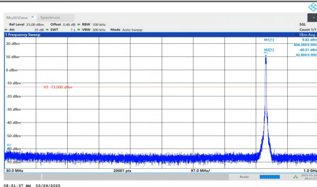
Band5-4182-30~1000MHz-PASS
