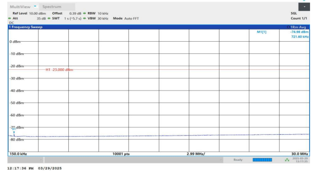
Band5-4132-2-0.15~30MHz-PASS
