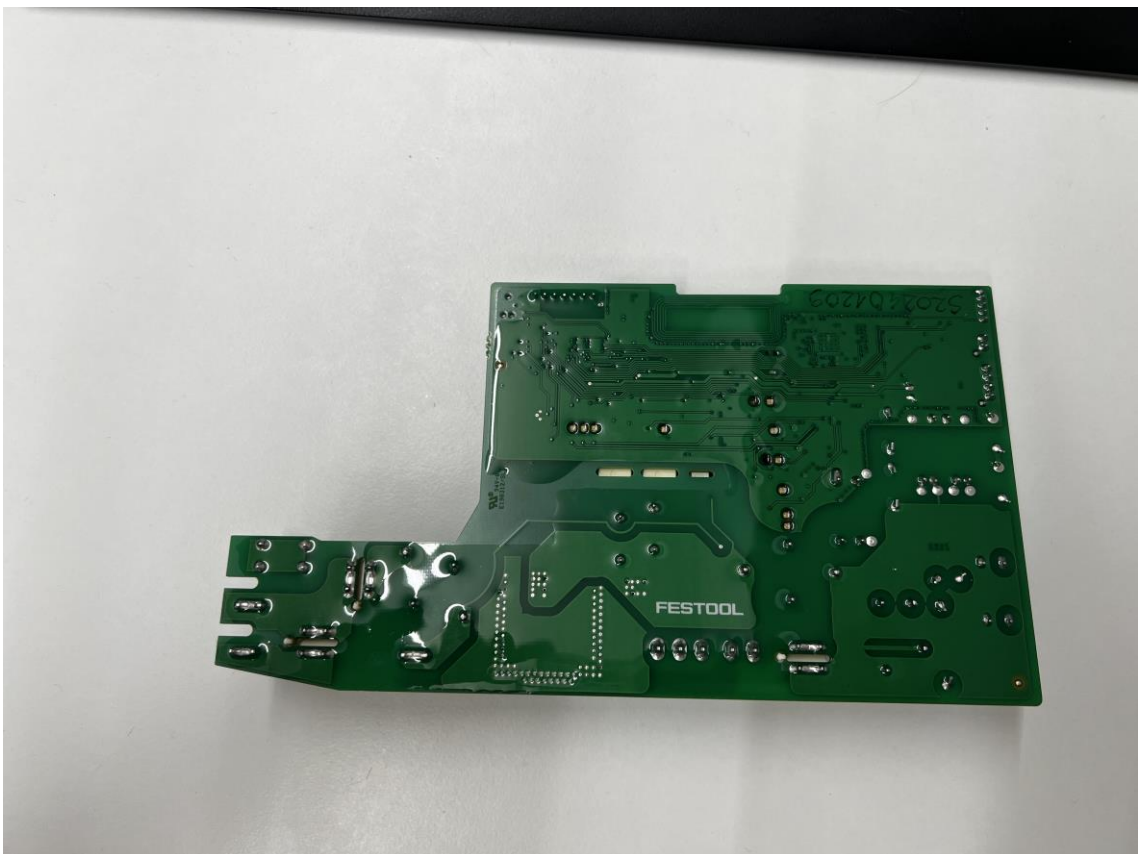
Figure 2: Back side of PCB
