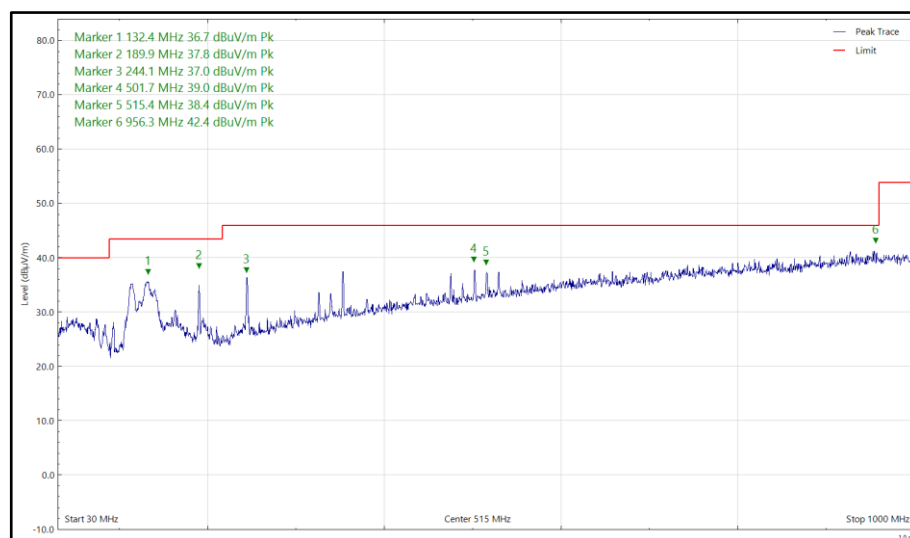
Figure 2 - NFC_BLE, 13.56 MHz_2402 MHz, 30 MHz to 1 GHz, Horizontal (Peak)
