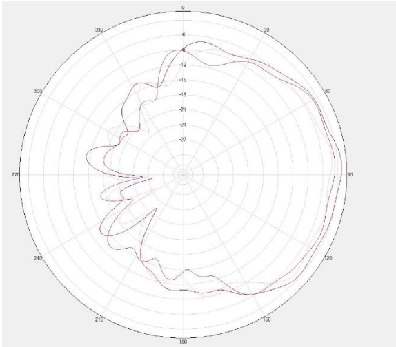
Phi=0 deg
