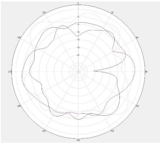
Phi=90 deg
