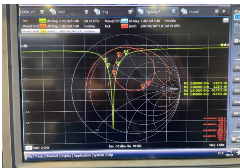
Figure 4.Return Loss
